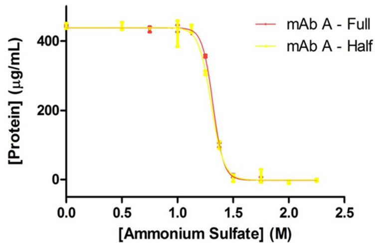
Figure 3. Solubility curve comparison of full and half volume assays. KBS assays show superimposable plots, and a AS m variance of 1.32 M for the full volume and 1.30 M for the half volume assay, or only 1.5% difference
