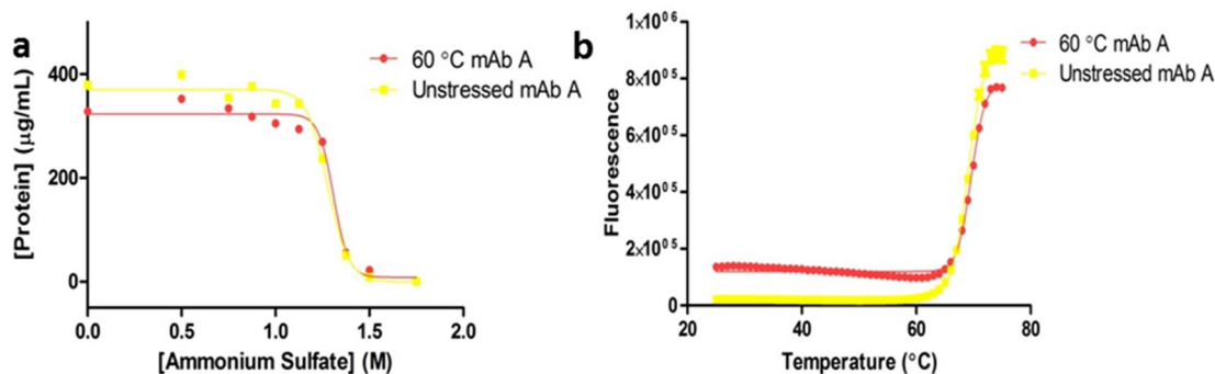
Figure 7. DSF and KBS evaluation of mAb subjected to extreme heat stress. MAb A was heat stressed at 60 °C for 15 hours, and evaluated by KBS and DFS. (a) The KBS assay shows very minor differences from the unstressed material, with a slightly lower maximum concentration, which could be caused by slightly lower starting concentration. (b) The T_m value of the super stressed material are minimally different from the control, however there is a 5-fold increase in the baseline fluorescence, suggesting an increase in the ambient hydrophobic environment.
