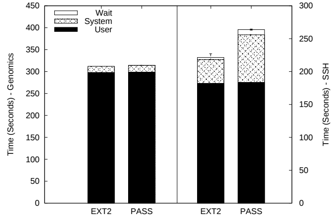
Figure 6: Overhead for Genomics workload and SSH Compile. The first half of the graph is the Genomics workload result and uses the left scale. The second half of the graph is the SSH Compile result and uses the right scale.
