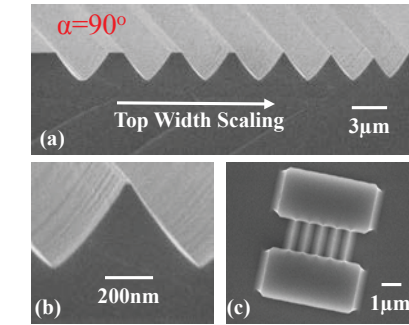
Fig. 8 (a) and (b) SEM cross-sectional illustration of wave structure formation by Ti mask width scaling. A triangular InGaAs structure is formed due to the anisotropic wet etching. (c) The top view of a fabricated InGaAs wave structure by the wet etching technology.
