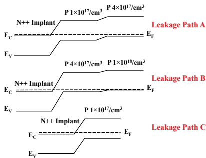
Fig. 23 Summary of energy barriers for possible off-state leakage paths of devices in this work. Leakage Path A is for InGaAs FinFET devices fabricated on substrate A. Leakage Path B is for InGaAs FinFET devices fabricated on substrate B. Leakage Path C is for InGaAs devices fabricated on substrate A but without mesa isolation.
