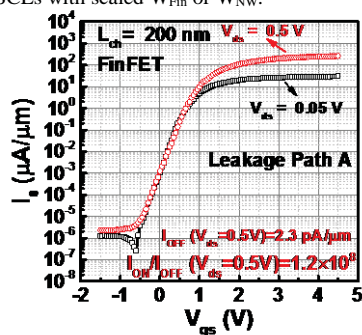
Fig. 22 Transfer characteristics of an InGaAs FinFET on bulk InGaAs with L_{ch}=200nm and record I_{ON}/I_{OFF}=1.2 \times 10^8 . The high I_{ON}/I_{OFF} is obtained by barrier engineering on the off-state leakage path.
