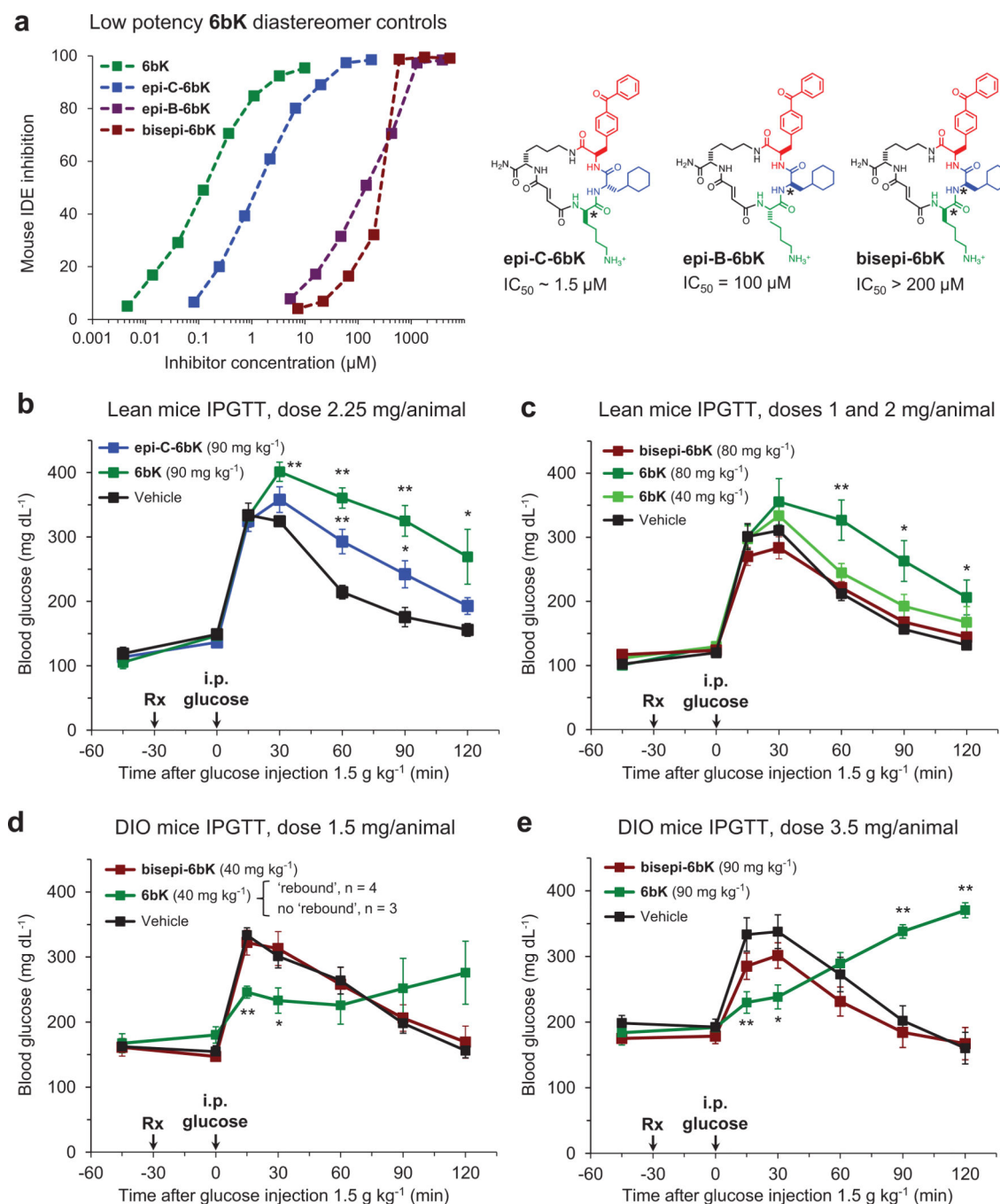
Extended Data Figure 7. Low-potency diastereomers of 6bK used to determine effective dose range and confirm on-target IDE inhibition effects during IPGTTs
