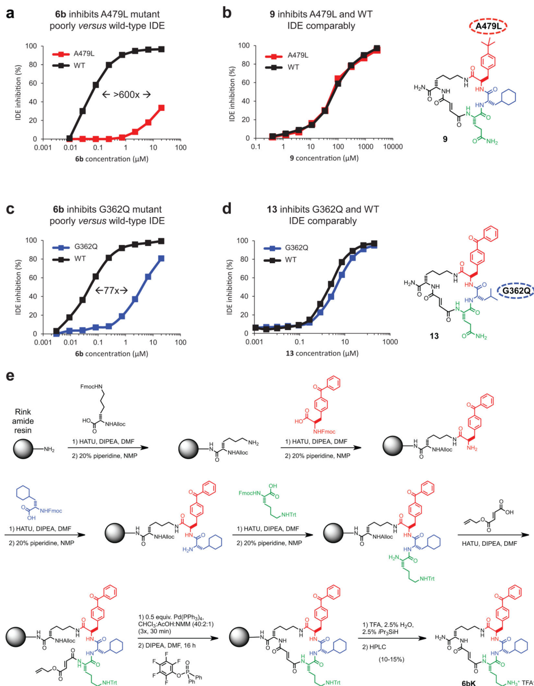
Extended Data Figure 4. Small-molecule/enzyme mutant complementation study to confirm the macrocycle binding site and placement of the benzophenone and cyclohexyl building-block groups
