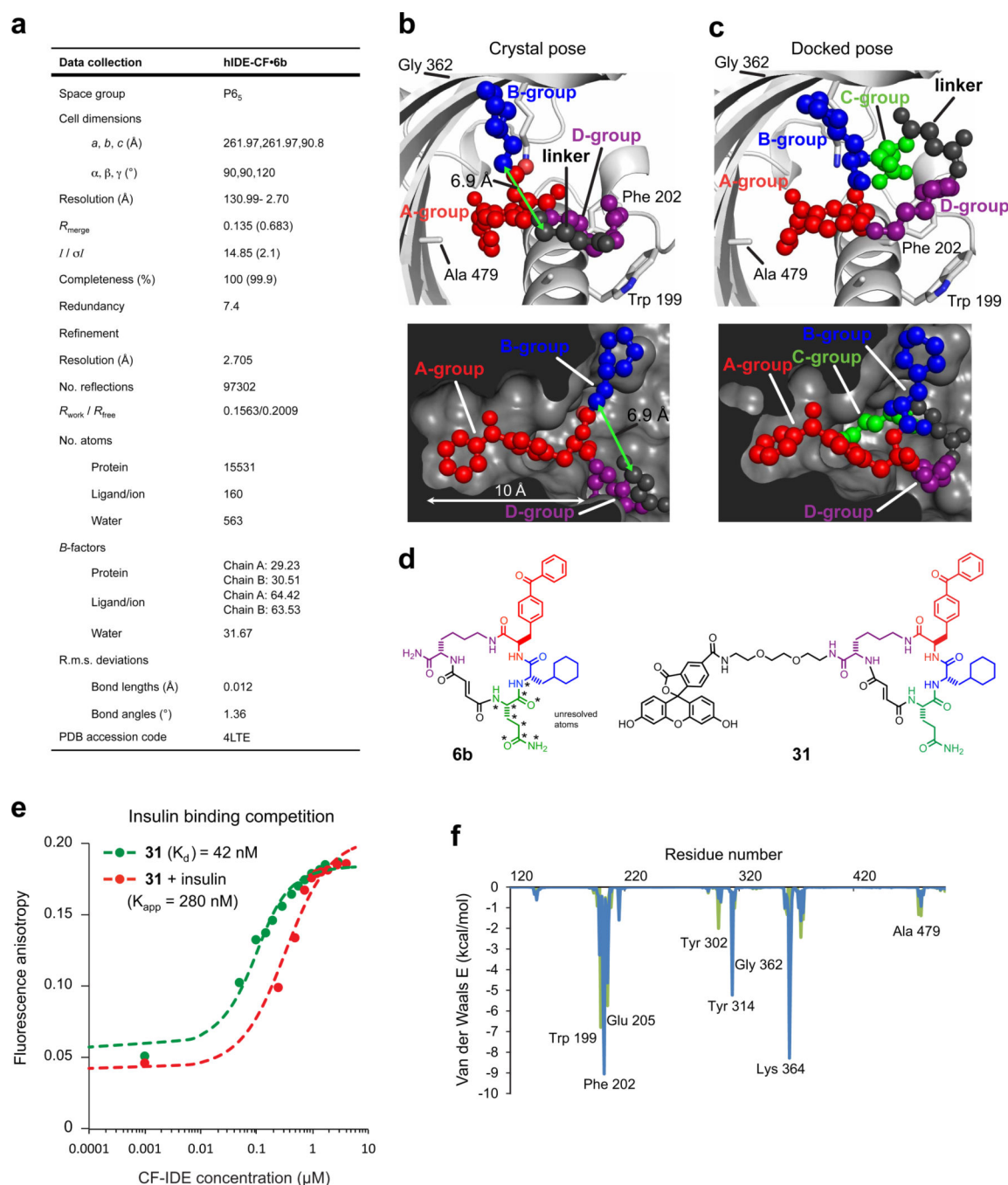
Extended Data Figure 3. Data collection and refinement statistics (molecular replacement), docking simulation for 6b, and competition test between insulin and fluorescein-labelled macrocycle 31 for binding cysteine-free IDE (CF-IDE)
