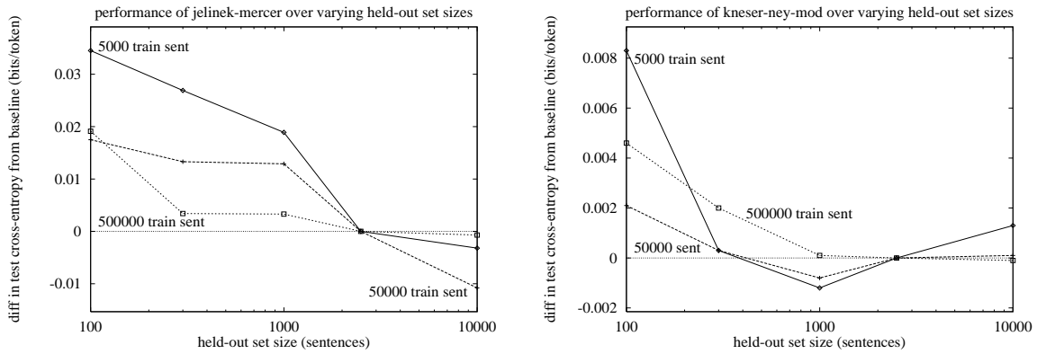
Figure 2: Performance relative to baseline held-out set size (2,500 sentences) of jelinek-mercer and kneser-ney-mod over several held-out set sizes; held-out set is used to optimize smoothing algorithm parameters
