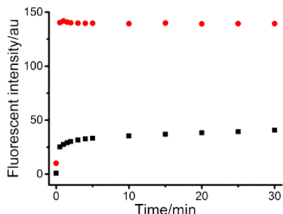
Figure 2. Time-dependent fluorescence changes of the probes ( 10\text{ }\mu\text{M} ) in the presence of \text{Na}_2\text{S} ( 50\text{ }\mu\text{M} ). The reactions were carried out for 30 min at room temperature in \text{CH}_3\text{CN}/\text{PBS} buffer (10 mM, pH 7.4, 1:1, v/v). Data were acquired at 455 nm with excitation at 340 nm for SeP1 (■) and at 521 nm with excitation at 498 nm for SeP2 (●).
