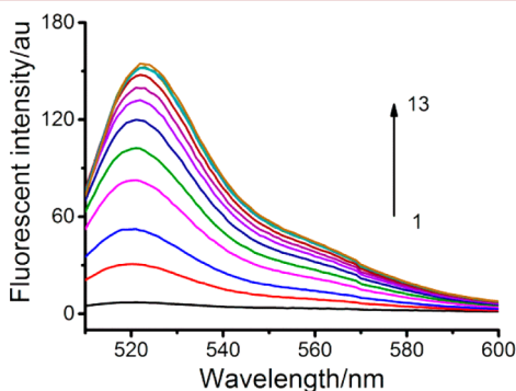
Figure 3. Fluorescence emission spectra of SeP2 ( 10\text{ }\mu\text{M} ) in the presence of varied concentrations of \text{Na}_2\text{S} (0, 0.5, 1, 2, 3, 4, 5, 6, 7, 8, 9, 10, 15 \mu\text{M} ). The reactions were carried out for 5 min at room temperature in \text{CH}_3\text{CN}/\text{PBS} buffer (10 mM, pH 7.4, 1:1, v/v). Data were acquired with excitation at 498 nm for SeP2 .
