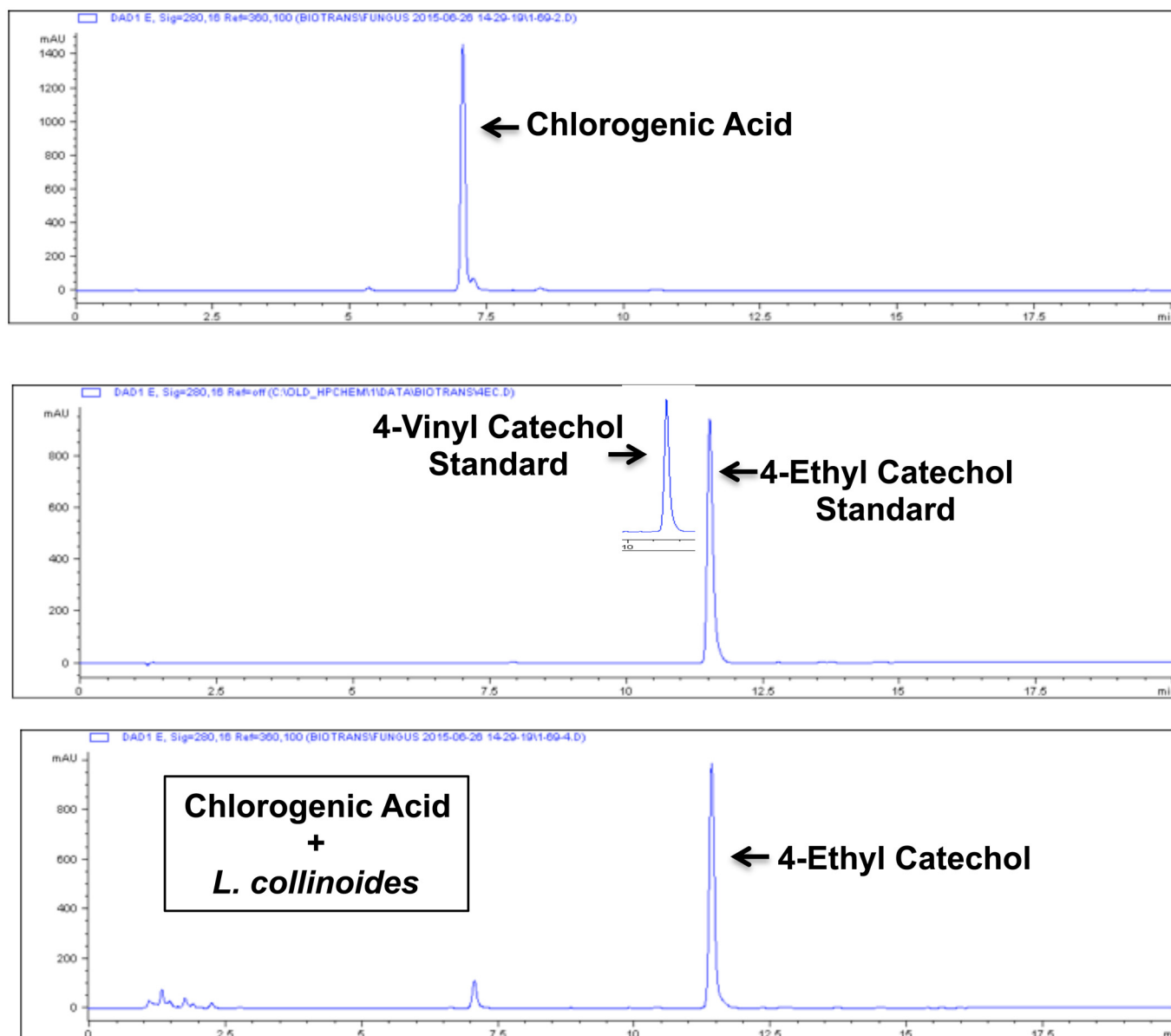
Fig 17. Biotransformation of chlorogenic acid by L. collinoides , as demonstrated with HPLC. Y-axis = absorbance at 254nm (mAU), X-axis = minutes. Top panel: HPLC of chlorogenic acid standard. Middle panel: HPLC of 4-vinylcatechol and 4-ethylcatechol standards. Bottom panel: HPLC of supernatant from chlorogenic acid + L. collinoides incubation, consistent with conversion of chlorogenic acid to 4-ethylcatechol. Retention times: chlorogenic acid = 7.1 minutes, 4-vinylcatechol = 10.7 minutes, 4-ethylcatechol = 11.6 minutes.
