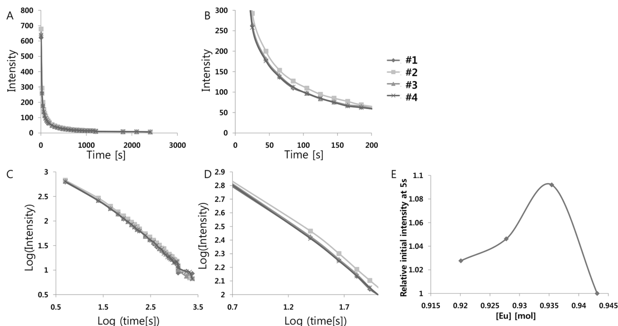
Fig 2. (A) Decay curves depending on Eu^{2+} concentration. (B) Magnified views of the graph in (A). (C) Decay curves in log scale depending on Eu^{2+} concentration. (D) Magnified views of the graph in (C). (E) Relative initial intensity measured at 5s (relative values where the value of control sample #1 is 1.0) depending on Eu^{2+} concentration.
