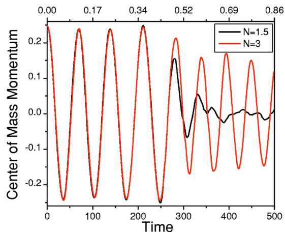
FIG. 10. Time dependence of the condensate momentum in a two-dimensional harmonic trap with different filling factors per central site.
