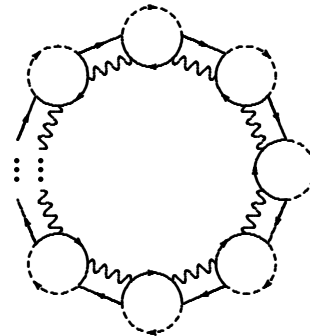
FIG. 3: The same as fig. 2 for a non-Abelian theory.
