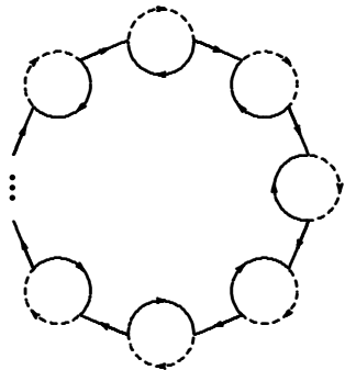
FIG. 2: The leading diagram contributing to the vacuum energy.
