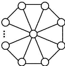
FIG. 5: A non-local theory space.
