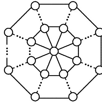
FIG. 6: Spider web theory space.
