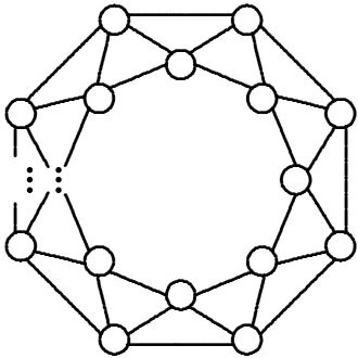
FIG. 4: Ribbon theory space
