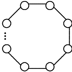
FIG. 1: Theory space for a U(1)^N model.
