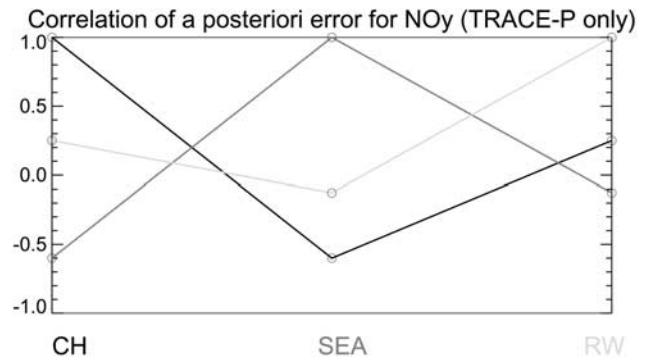
Figure 11. Individual rows of the correlation matrix for the inversion of NO y sources using only the TRACE-P aircraft data. Different colors distinguish rows of the matrix, with the corresponding columns indicated on the x axis. Lines connect the symbols for clarity and do not have any physical significance. See color version of this figure at back of this issue.
