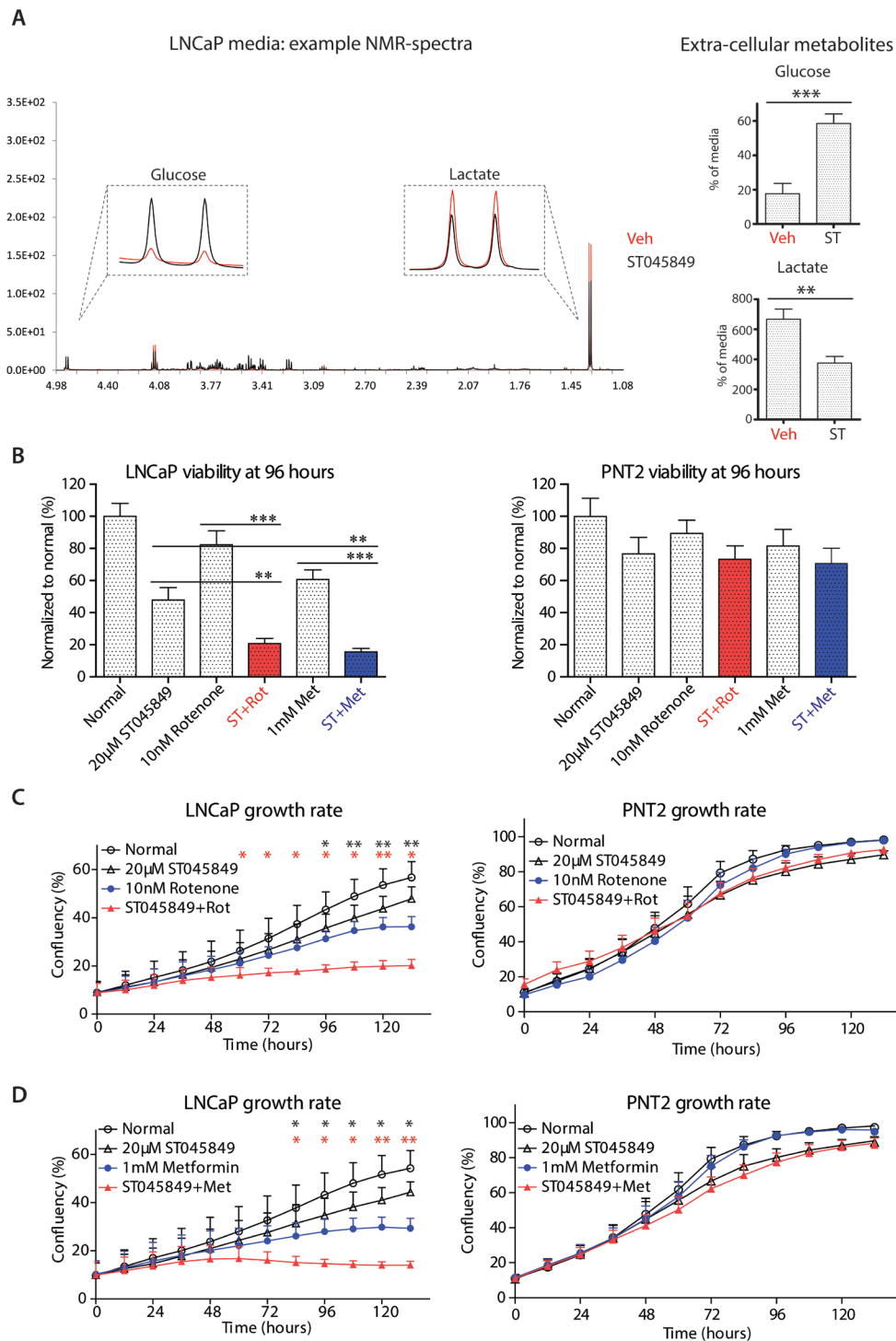
Figure 2: Metabolomic profiling of cell culture media after OGT inhibitor ST045849 treatment. A. LNCaP cells were treated with 20µM OGT inhibitor ST045849 for 96 hours, cell media were collected and analyzed by ^1\text{H} NMR. An example of the obtained NMR spectra is shown. The levels of glucose and lactate were determined from the cell culture media by ^1\text{H} NMR. The data shown is an average of seven biological replicates with SEM. The significance was assessed with Student's t -test, ** < 0.01 , *** < 0.001 . B. Cells were treated as indicated in the figure and the viability of cells was analysed with CTG reagent after 96 hours treatment. Viability of the untreated sample was set to 100% and treatments were normalized to this. The data shown is an average of four biological replicates with SEM. The significance was assessed with Student's t -test, ** < 0.01 , *** < 0.001 . C. and D. Cells were treated as indicated in the figure and the growth rate of cells was recorded by life cell imaging. The data shown is an average of four biological replicates with SEM. The significance was assessed with Student's t -test, * < 0.05 and ** < 0.01 . Black stars indicate comparison between rotenone (or metformin) only and combination of ST045849 with rotenone (or metformin), while red stars indicate comparison between ST045849 and combinatorial treatments.
