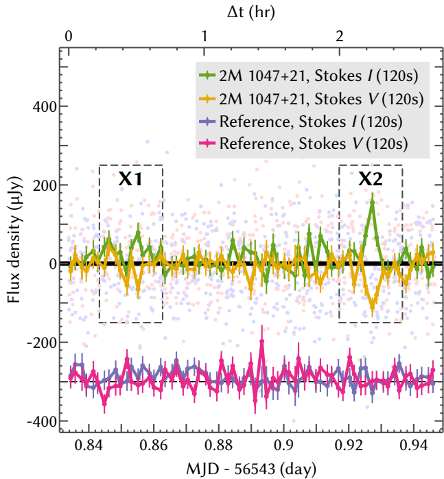
Figure 2. Stokes I and V radio light curves of 2M 1047+21 and a reference source (offset for legibility) in the 9–11 GHz spectral window. Symbols and colors are as in the top panel of Figure 1 . Uncalibrated polarimetric leakage terms introduce additional \lesssim 10\% systematic uncertainties into the flux measurements.
