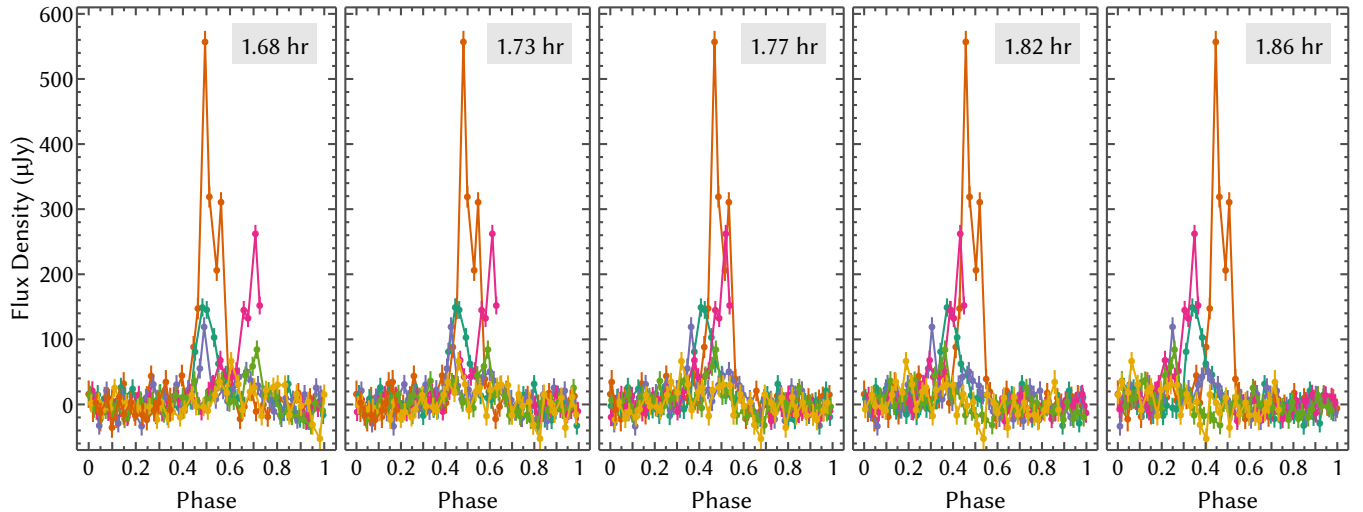
Figure 3. Frequency-averaged \overline{I-V} light curve of 2M 1047+21 , phased with different periodicities (labeled within each panel). The central panel phases at the best PDM periodicity of 1.77 hr.
