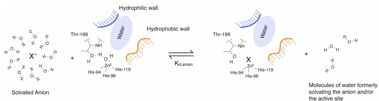
Figure 7. Anion-protein association in aqueous solution. Weakly hydrated Hofmeister anions can associate with the Zn 2+ cofactor of human carbonic anhydrase II (HCAII). The free energy of binding is influenced by rearrangements in the water surrounding the anion and filling the binding pocket of the protein. This figure is reproduced with permission from reference [82] .
