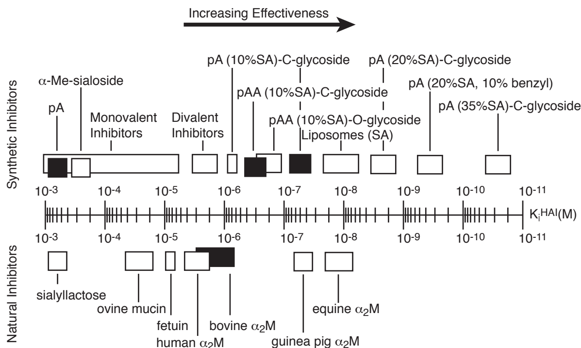
Figure 6. Constants K^{HAI} describing the inhibition, by a derivative of sialic acid, of the clumping of chicken erythrocytes caused by influenza virus. (This clumping process is believed to mimic an early step in the entry of influenza virus into mammalian cells—that is, the association of the virus with the cell via attachment of one or more trimers of hemagglutinin on the surface of the virus to sialic acid groups on the surface of the cell). Each sialic acid included in a copolymer of acrylamide and acrylamide covalently linked to sialic acid is 10^9 more effective at inhibiting cell clumping than is \alpha -methylsialoside. ( \alpha_2 M is \alpha_2 Macroglobulin.) We elaborate on the use of sialosides in the design of polyvalent inhibitors of the influenza-mediated clumping of cells in reference [111].
