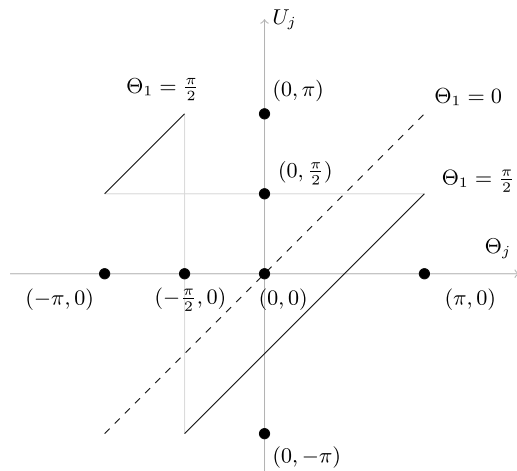
FIG. 1. For every value of \Theta_1 \neq 0 , the map \Theta_j \mapsto U_j ( j \geq 2 ) is a disjoint union of two lines, and is one-to-one. The figure shows the graph of (\Theta_j, U_j) when \Theta_1 = \frac{\pi}{2} (plotted as two solid lines). When \Theta_1 = 0 , U_j = \Theta_j (plotted in dashed line).
