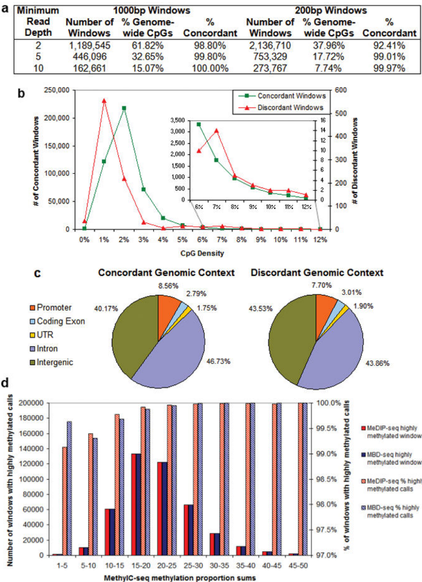
Figure 3. Comparison of methylated DNA enrichment methods (a) Calls of highly/weakly methylated were made by averaging methylation scores for CpGs covered at varying minimum read depths by MeDIP-seq or MBD-seq in 1000bp and 200bp windows. The number of windows, percent of genome-wide CpGs covered, and the percent of concordant calls are shown for each minimum read depth and window size. For the 1000bp windows with a minimum read depth of 5, the (b) CpG density and (c) genomic context of the concordant and discordant windows are shown. The inset in (b) shows a close-up of the concordance/discordance of CpG densities consistent with CGIs. (d) For the 1000bp windows with a minimum read depth of 5, MethylC-seq methylation proportions for CpGs and non-CpG cytosines covered at a minimum read depth of 5, 444,590 windows, were summed and the windows were binned by the sum. For each of these bins, the number of windows called highly methylated by MeDIP-seq or MBD-seq is shown on the left y-axis
