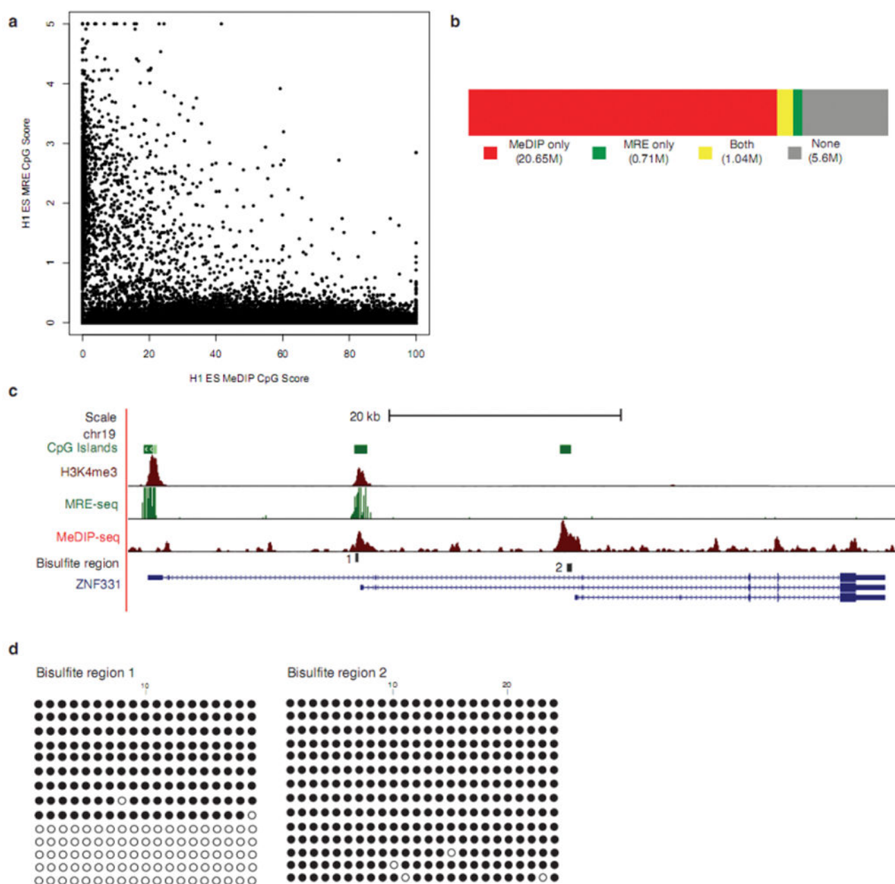
Figure 5. Integrative method increases methylome coverage and enables identification of a DMR (a) MRE-seq involves parallel digests with methylation sensitive restriction enzymes (HpaII, AciI, and Hin6I), selection of cut fragments of approximately 50bp–300bp, pooling the digests, library construction, and sequencing. For every 600bp window along chromosome 21, MeDIP-seq scores were plotted against MRE-seq scores. The plot depicts the inverse relationship between MRE-seq and Me-DIP-seq signals. (b) Coverage of CpGs in the human genome by MeDIP-seq alone (red), MRE-seq alone (green), both (yellow), or neither method (no fill). Sequence from replicate #1 and #2 were used in these calculations (c) UCSC Genome Browser view of ZNF331 in H1 ESC, showing overlap of Me-DIP-seq, MRE-seq and H3K4me3 (from ChIP-seq) signals at bisulfite region 1 and only MeDIP-seq
