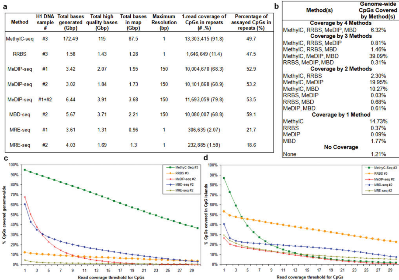
Figure 1. Critical parameters in sequencing-based DNA methylation profiling Sequencing statistics and CpG coverage are shown for MethylC-seq, (207 lanes, data analyzed here were from Lister, et al. 8.), RRBS (2 lanes), MeDIP-seq (4 lanes each), MBD-seq (3 lanes), and MRE-seq (3 lanes each). Since the amount of sequence produced per lane is increasing, we also provide “Gbp of sequence” as a measure of the relative cost of each method. The methods differ significantly in total bases generated by the Illumina sequencer, total high quality bases passing Illumina chastity filtering and mapping uniquely, and total bases used for generating methylome maps (high quality bases passing redundancy filters) (a) The H1 replicates assayed and the Gbp of sequence at successive processing stages by each method are shown. The bisulfite-based methods and MRE-seq resolve the methylation status of individual cytosines, whereas the MeDIP-seq and MBD-seq read mappings are extended to 150bp, resulting in a maximum resolution of 150bp. This extension is applied to calculations of CpG coverage but is not applied to the Gbp of sequence at the processing stages. Coverage information is shown for repeats (primarily transposon sequences) genome-wide. While maximum resolution of each method is reported, resolution can be assessed at various levels. As the level of resolution decreases, as a consequence of averaging of methylation scores over a window of larger size for example, imperfect coverage and limited accuracy become less limiting, provided that the average score is not affected by systematic biases in coverage and accuracy. Thus, methylome coverage and
