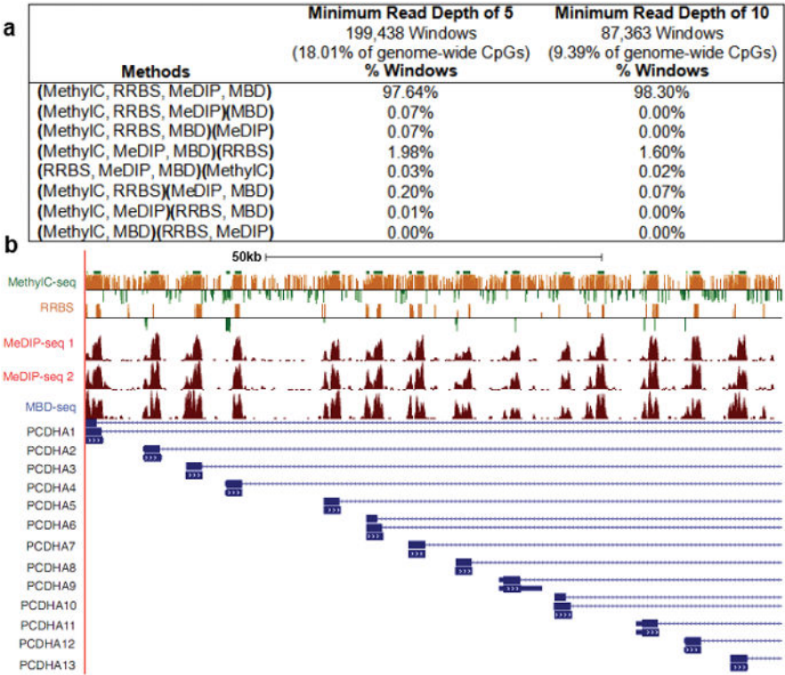
Figure 4. Comparison of all methods (a) The table shows the percentage of 1000bp windows with concordant and discordant MethylC-seq (replicate #3), RRBS (replicate #3), MeDIP-seq (replicate #2) and MBD-seq (replicate #2) calls at minimum read depths of 5 and 10. Methods making the same call are grouped together in parentheses. Calls were made for MethylC-seq and RRBS by averaging the methylation proportion of CpGs within the window that were covered at the minimum read depth and applying a highly/weakly methylated cutoff of 0.2. Calls were made for MeDIP-seq and MBD-seq by averaging the methylation score of CpGs within the window that were covered at the minimum read depth. (b) Genome browser view of the 100kb CpG rich Protocadherin alpha cluster (PCDHA) exemplifying the significant concordance in methylation status seen on a genome-wide level. For Methyl-seq and RRBS, the Y- axis displays methylation scores of individual CpGs. Scores range between -500 (unmethylated) and 500 (methylated), and the zero line is equivalent to 50% methylated. Negative scores are displayed as green bars and positive scores are displayed as orange bars. For MeDIP-seq 1, MeDIP-seq 2 and MBD-seq, the Y-axis indicates extended read density. Browseable genome-wide views of these datasets are available at http://www.genboree.org and http://genome.ucsc.edu/ .
