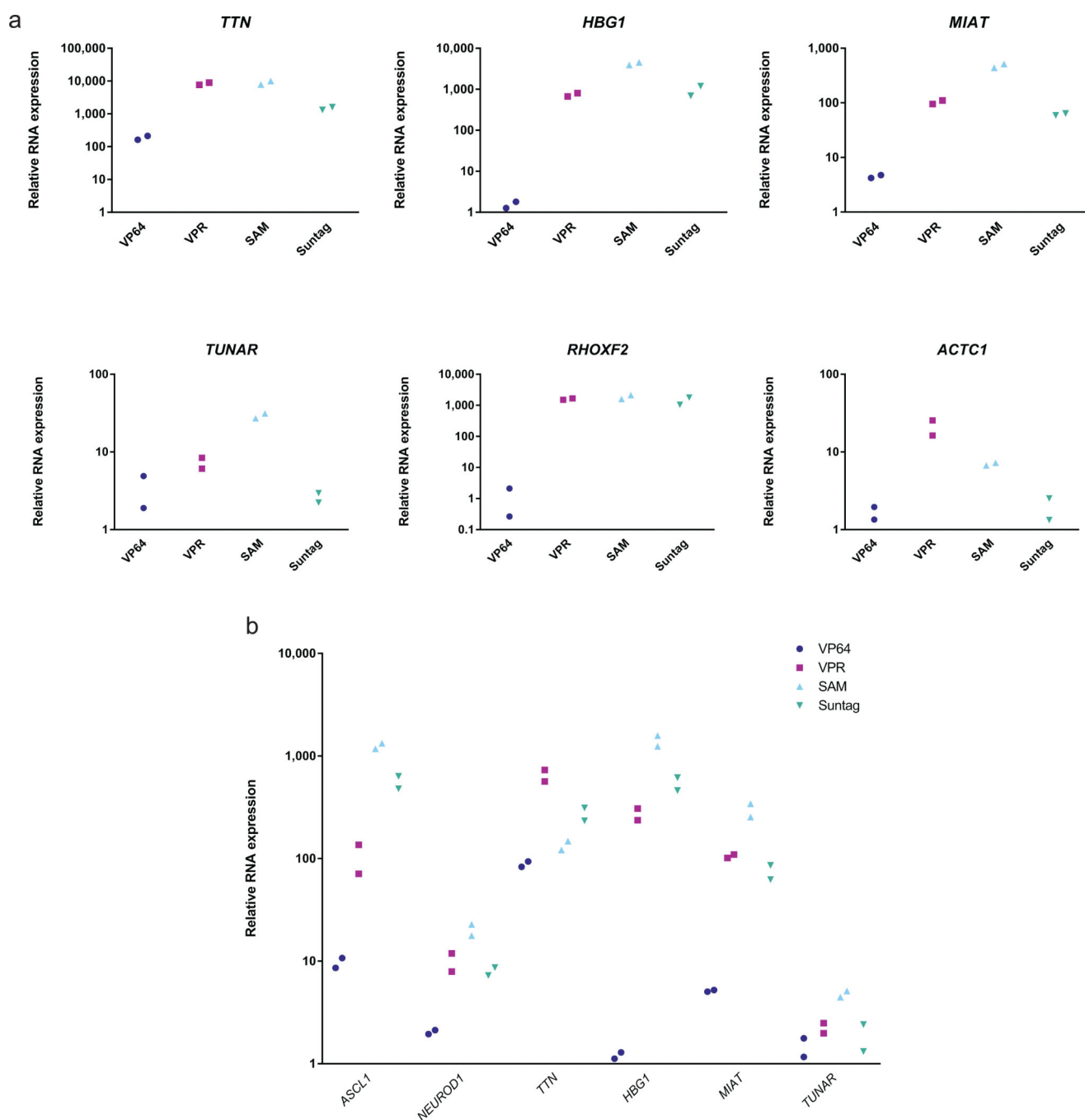
Figure 2. Activation of endogenous genes in HEK 293T cells
