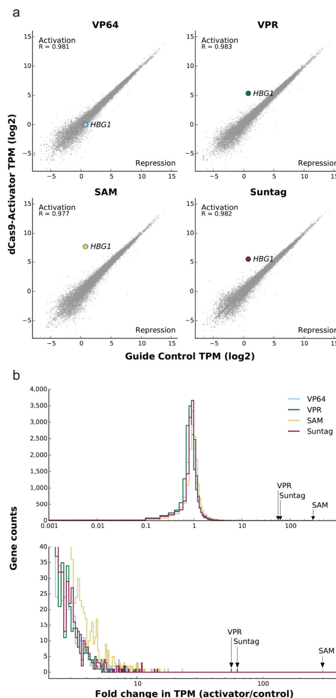
Figure 3. Evaluation of activator specificity by RNA sequencing
