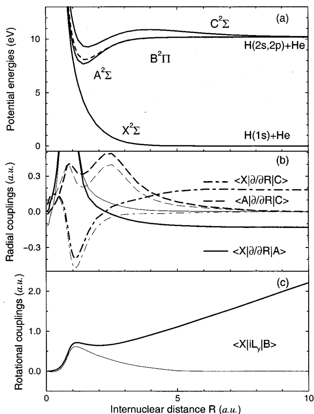
FIG. 4. The adiabatic potentials (a), the radial (b), and the rotational (c) couplings for the HeH system calculated with the origin of the electron coordinates at the center of nuclear mass (thick lines) and at the proton (thin lines).
