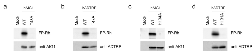
Figure 2. Identification of Thr and His residues critical for FP labeling of AIG1 and ADTRP. (a-d) ABPP gels and Western blots of membrane proteomes ( 0.5 \text{ mg proteome mL}^{-1} ) showing selective FP-Rh labeling of WT-, but not the indicated Thr-to-Ala and His-to-Ala mutants of human (h) AIG1 (a, c) and ADTRP (b, d) in transfected HEK293T cell lysates. Proteomes were treated with 1 \text{ }\mu\text{M} FP-Rh for 30 min at 37 \text{ }^{\circ}\text{C} . Full images of gels and Western blots are provided in Supplementary Figure 16 .
