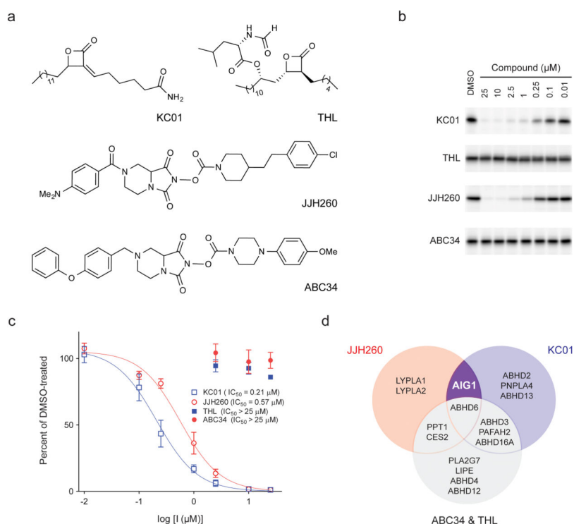
Figure 4. Discovery of inhibitors and structurally related inactive control compounds for AIG1. (a) Chemical structures of two hAIG1 inhibitors, KC01 and JJH260, and the respective control compounds, THL and ABC34. (b) ABPP gels demonstrating inhibition of FP-Rh labeling of hAIG1 by KC01 and JJH260, but not THL and ABC34. Proteomes were treated with each inhibitor at the indicated concentrations for 30 min at 37 °C, followed by FP-Rh (1 μM, 30 min, 37 °C). Full images of the gels are provided in Supplementary Figure 18 . (c) Concentration-dependent inhibition of the 9-PAHSA hydrolysis activity of hAIG1-transfected HEK293T membrane proteome by KC01 ( IC_{50} = 0.21 \pm 0.08 \mu M ) and JJH260 ( 0.57 \pm 0.14 \mu M ), but not THL and ABC34. For these experiments, proteomes were incubated with each inhibitor at the indicated concentration for 30 min at 37 °C. 20 μg of each proteome was then incubated with 100 μM 9-PAHSA for 30 min at 37 °C. Data represent mean values \pm s. e. m. for three biological replicates. (d) Venn diagram showing overlapping and distinct target profiles for AIG1 inhibitors KC01 and JJH260 and control compounds THL and ABC34.
