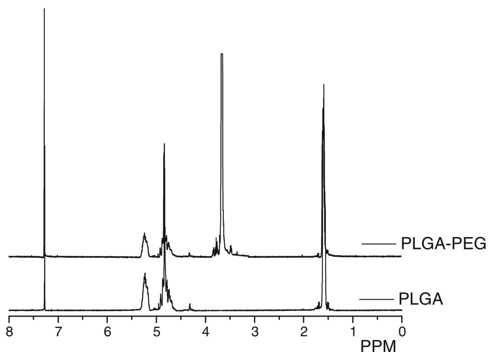
Fig. 1. PLGA- b -PEG characterization using nuclear magnetic resonance (NMR). The presence of PLGA and PEG were visualized in using a 400 MHz ^1\text{H} NMR ppm 5.2 (m, ((\text{OCH}(\text{CH}_3)\text{C}(\text{O})\text{OCH}_2\text{C}(\text{O}))_n-(\text{CH}_2\text{CH}_2\text{O})_m) , 4.8 (m, ((\text{OCH}(\text{CH}_3)\text{C}(\text{O})\text{OCH}_2\text{C}(\text{O}))_n-(\text{CH}_2\text{CH}_2\text{O})_m) , 3.7 (s, ((\text{OCH}(\text{CH}_3)\text{C}(\text{O})\text{OCH}_2\text{C}(\text{O}))_n-(\text{CH}_2\text{CH}_2\text{O})_m) , 1.6 (d, ((\text{OCH}(\text{CH}_3)\text{C}(\text{O})\text{OCH}_2\text{C}(\text{O}))_n-(\text{CH}_2\text{CH}_2\text{O})_m) (reproduced from ref. (7) with permission from PNAS, Copyright (2008) National Academy of Sciences, U.S.A.).
