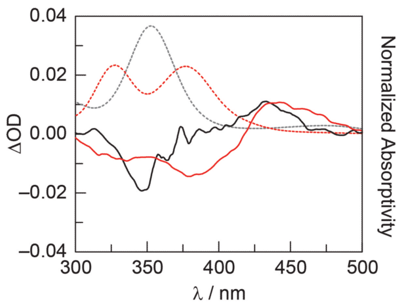
Fig. 4. Transient absorption spectra obtained by laser flash photolysis ( \lambda_{\text{exc}} = 355 nm) of complexes 1 (solid red) and 2 (solid black), respectively. Spectra are normalized to the absorbance at \sim 440 nm. Normalized absorption spectra of 1 (dashed red) and 2 (dashed black) are also shown
