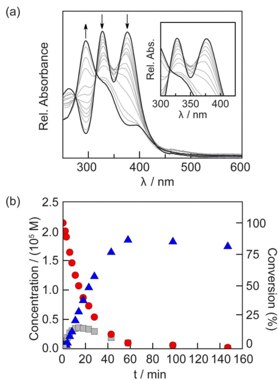
Fig. 2. (a) Spectral evolution during photolysis of Rh 2 [I,III] complex 1 in THF. Inset: Expanded spectrum to show that isosbestic points are not observed, consistent with evolution of a steady-state intermediate during the photolysis of 1 . (b) Concentration profiles of 1 (red circle), 2 (gray square) and 3 (blue triangle) during the photolysis of 1 .
