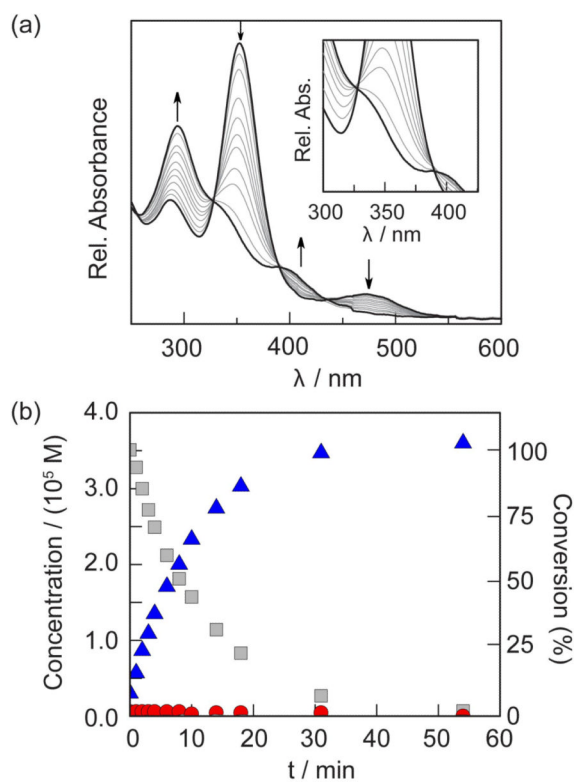
Fig. 3. (a) Spectral evolution during photolysis of Rh 2 [II,II] complex 2 in THF. Inset: Expanded spectrum to show that isobestic points are observed, precluding a steady-state intermediate. (b) Concentration profiles of 1 (red circle), 2 (gray square) and 3 (blue triangle) during the photolysis of 2 .
