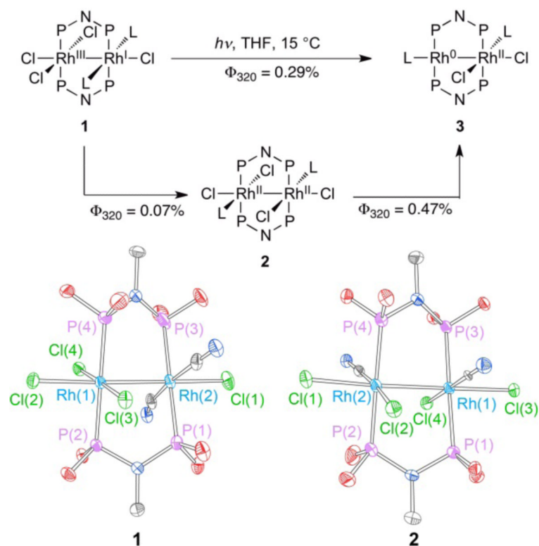
Fig. 1. Photolysis of two-electron mixed-valent \text{Rh}_2[\text{I},\text{III}] complex 1 affords \text{Rh}_2[0,\text{II}] complex 3 via both direct halogen elimination, as well as isomerization to valence-symmetric \text{Rh}_2[\text{II},\text{II}] 2 , which undergoes halogen elimination; L = 1-adamantylisocyanide, P–N–P = bis (trifluoroethoxy)phosphinylmethylamine (tfepma). Thermal ellipsoid plots of 1 and 2 drawn at the 50% probability level. The -\text{CH}_2\text{CF}_3 , adamantyl groups and hydrogen atoms are omitted for clarity.
