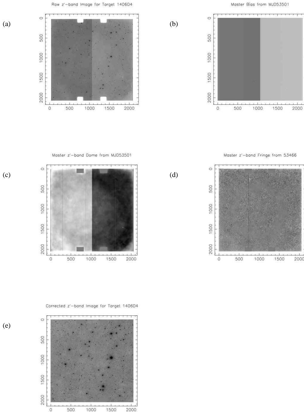
Fig. 5 The image processing steps, using PT data from MJD 53501 as an example: (a) the raw z' -band image of the secondary patch 1406D4, (b) the master bias frame from MJD 53501, (c) the master z' -band dome flat from MJD 53501, (d) master z' -band fringe frame from MJD 53466 (used for processing the PT data from MJD 53501), (e) the bias-subtracted, trimmed, flat-fielded, and fringe-corrected z' -band image of the secondary patch 1406D4. The (linear) stretch used in these images is from 90% to 110% of the given image's median pixel value.
