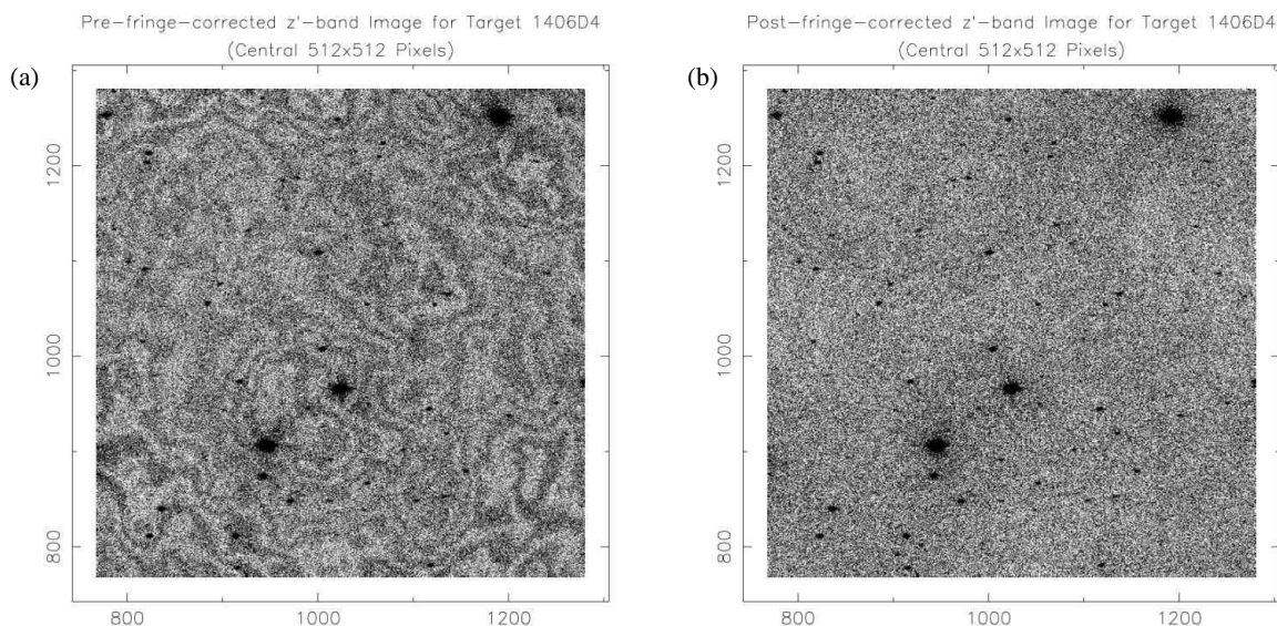
Fig. 6 An example of de-fringing a PT z' -band image: (a) the central 512 \times 512 pixels of the bias-subtracted, trimmed, flat-fielded, but not fringe-corrected z' -band image of the field featured in Figure 5; (b) the same as (a), but after fringe-correction. The (linear) stretch in these two images is the same (from 95% to 105% of the median pixel value of (a)). The typical trough-to-peak amplitudes of the fringes in (a) is \approx 2\% .
