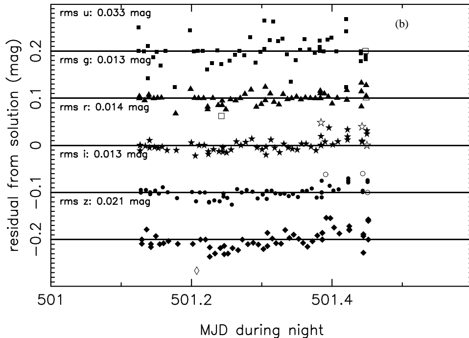
Fig. 8 A sampling of the quality assurance plots output by excal for the PT data taken on the night of MJD 53501: (a) first-order extinctions ( k coefficients) vs. time for each of the five passbands, and (b) magnitude residuals for the u'g'r'i'z' standard stars observed over the course of the night (the zero lines are staggered by 0.1 mag offsets in order to include the residuals from all five filters on the same plot). Note that, in (b), solid symbols denote the observations that were included in the solution, whereas open symbols denote the observations that were removed from the solution.
