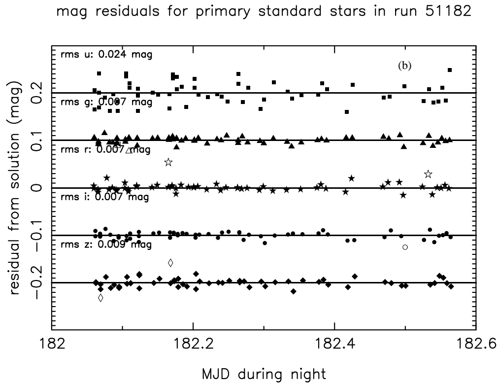
Fig. 9 The same exca.l quality assurance plots as in Figure 8, but for the USNO-1.0m data taken on the night of MJD 51182, in which the k terms were solved for in 3-hour time blocks.
