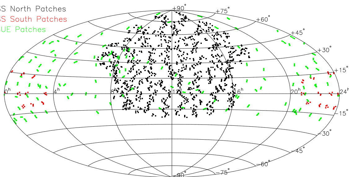
Fig. 2 Locations of the SDSS secondary patches in equatorial coordinates (Aitoff projection): ( black ) Northern SDSS patches, ( red ) Southern SDSS patches, and ( green ) SEGUE patches. (SEGUE is part of the Sloan extension, or SDSS-II, and is discussed in § 5.)
