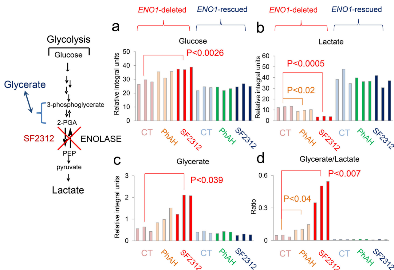
FIGURE 5. SF2312 selectively blocks glycolysis in ENO1-deleted glioma cells
