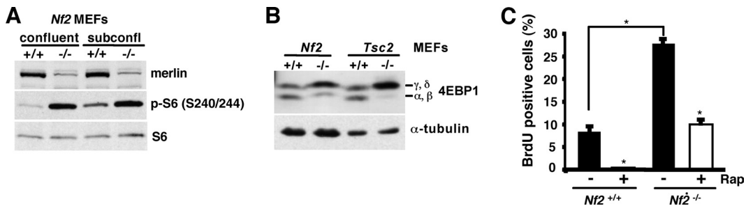
FIG. 7. Nf2 -deficient ( Nf2 -/- ) MEFs exhibit constitutive mTORC1 activation compared to Nf2 WT ( Nf2 +/+ ) MEFs. (A) Nf2 -/- MEFs, plated confluent and subconfluent (subconfl), exhibit constitutive S6 activation, in contrast to Nf2 +/+ MEFs, under conditions of serum starvation (0% FBS). (B) Nf2 -/- MEFs and Tsc2 -/- MEFs exhibit increased accumulation of phosphorylated species of 4EBP1 compared to that in control Nf2 +/+ and Tsc2 +/+ MEFs, respectively, under conditions of serum starvation (0% FBS). 4EBP1 phosphorylation (detected by anti-4EBP1 antibody) is reflected by 4EBP1 electrophoretic mobility results. (C) Rapamycin (Rap) suppresses the proliferation of Nf2 -/- MEF cells. Nf2 +/+ and Nf2 -/- MEFs incubated with 20 nM rapamycin or vehicle (DMSO) for 24 h were examined for S-phase entry by using BrdU incorporation as detailed in Materials and Methods. Data are presented as mean percentages of DAPI-stained cells ± standard errors of the means. *, P < 0.01 for DMSO-treated control versus rapamycin-treated groups or Nf2 +/+ versus Nf2 -/- MEF cells ( n = 5); +, present; -, absent.
