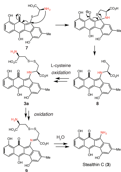
Scheme 1. Proposed mechanism for stealthin C formation.
