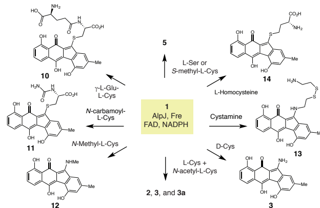
Figure 4. Reactivity of AlpJ-derived intermediates toward alternate nucleophiles.
