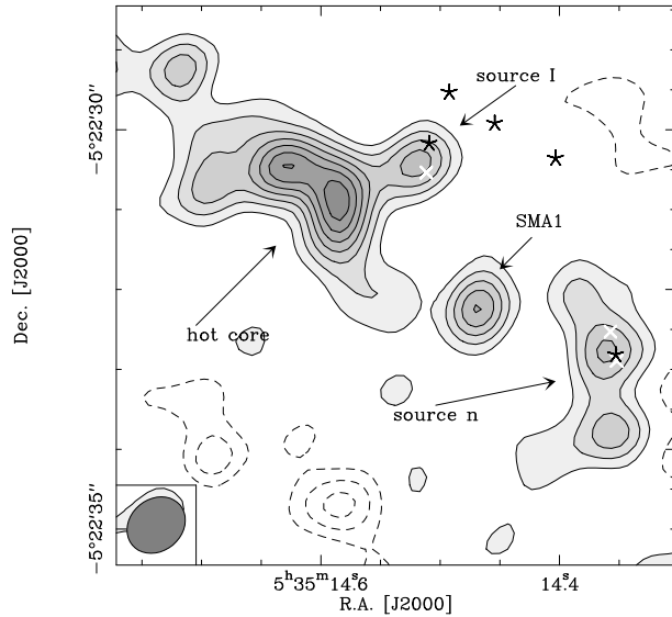
Fig. 1.— Sub-mm continuum image of the Orion-KL region at 865\ \mu\text{m} . The contouring starts at the 2\sigma level of 70\ \text{mJy}/\text{beam} and continues in 2\sigma steps. Positive emission is shown in grey-scale with contours, negative features – mainly due to missing flux – are presented in dashed contours. The white crosses mark the radio positions of sources I and n (two crosses for n because of the bipolar structure) (Menten & Reid 1995). The black stars mark the positions of emission peaks at 3.8\ \mu\text{m} (Dougados et al. 1993), rotated to the J2000 frame and corrected to account for the proper motion of BN (e.g., Plambeck et al. 1995; Tan 2004), which was used as an astrometry reference in near-infrared observations (position uncertainties are 0.03'' - 0.05'' ). The beam is shown at the bottom left ( 0.78'' \times 0.65'' ).
