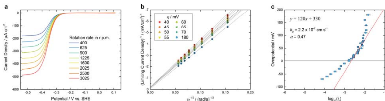
Figure S2. (a) Plot of potential vs. current density at different rotation rates of the rotating disk electrode (RDE). The solution is 1.00 mM BTMAP-Vi and 0.50 M NaCl in \text{H}_2\text{O} . Rotation rates are indicated. (b) Koutecký-Levich plot ( i^{-1} vs. \omega^{-1/2} ) of 1.00 mM BTMAP-Vi and 0.50 M NaCl in \text{H}_2\text{O} . The current response, i^{-1} , is shown for eight different BTMAP-Vi reduction overpotentials \eta . (c) Fit of RDE experimental data to the Butler-Volmer equation constructed using the current response in the absence of mass transport limitations at high BTMAP-Vi reduction overpotentials; i_k is the current extrapolated from the zero-intercept of the fitted lines in (b) (i.e. at infinite rotation rate). The line of best fit to the region between an overpotential of 40 – 80 mV has the equation y = 120x + 330 , from which \alpha = 0.47 and k_0 = 2.2 \times 10^{-2} \text{ cm s}^{-1} were calculated. Data were averaged over three runs.
