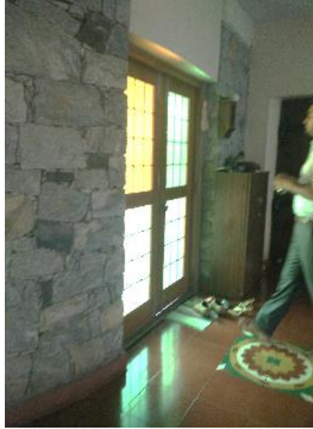
Figure 22. House 3 walls constructed with rubble masonry and no plaster.
