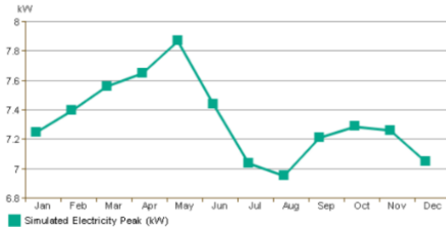
Figure 68. Existing house estimated monthly peak demand for house 5.
