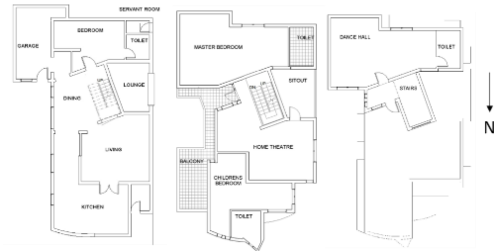
Figure 70. Floor plan of house 6. ground floor (left), first floor (center), second floor (right).
