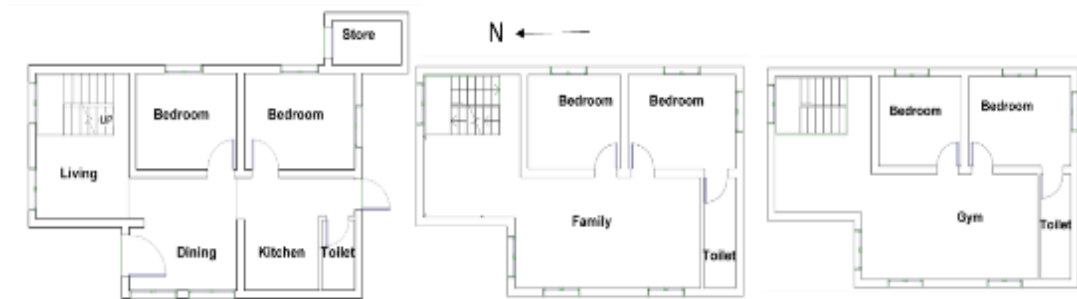
Figure 63. Floor plan for house 5. ground floor (left), first floor (center), second floor (right).
