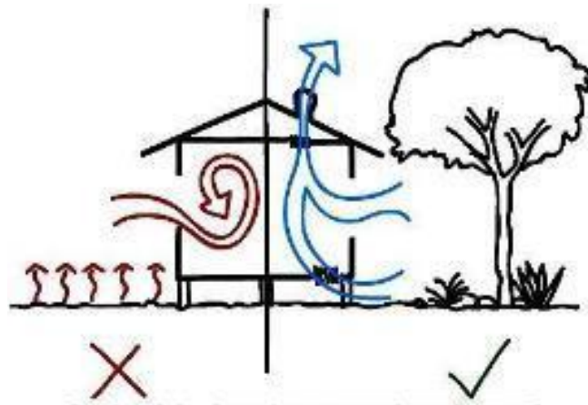
Figure 19. Section showing how clear story windows benefit air movement (Anderson, 2012). On the right, hot air escapes through a roof vent and draws cool air in convection. On the left, a lack of ventilation contributes to the stagnation of hot air.
