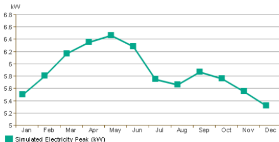
Figure 61. Existing house estimated monthly peak demand for house 4.
