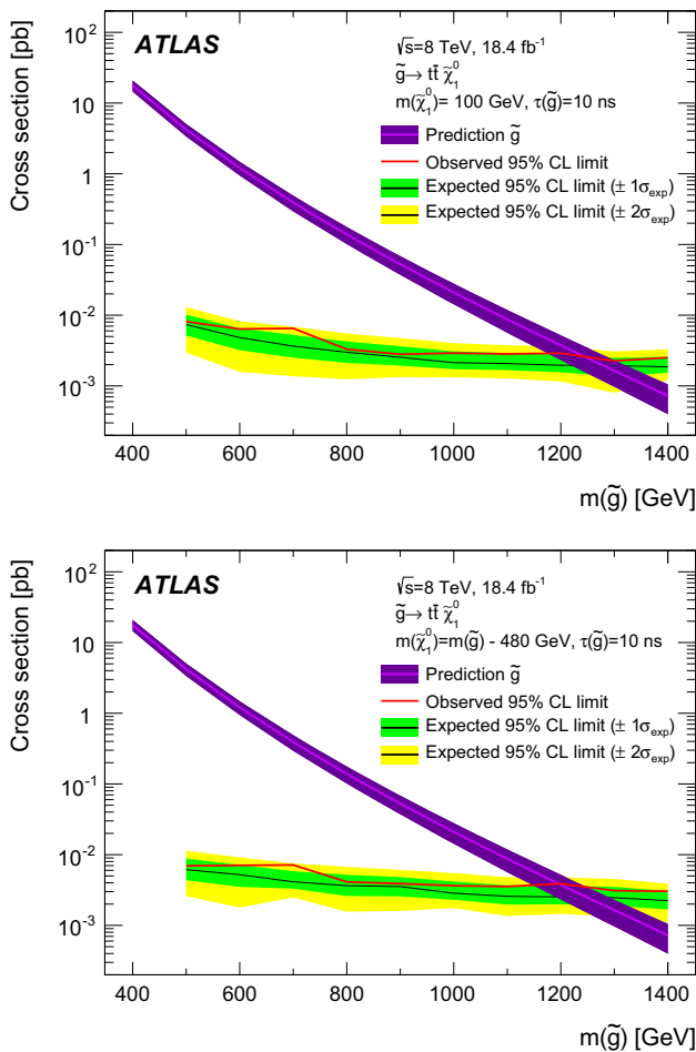
Fig. 8 Upper limits on the production cross section as a function of mass for metastable gluino R -hadrons, with lifetime \tau = 10\text{ ns} , decaying into t\bar{t} plus a light neutralino of mass m(\tilde{\chi}_1^0) = 100\text{ GeV} (top) or a heavy neutralino of mass m(\tilde{\chi}_1^0) = m(\tilde{g}) - 480\text{ GeV} (bottom). Theoretical values for the cross section are shown with their uncertainty. The expected upper limit in the background-only case is shown as a solid black line, with its \pm 1\sigma and \pm 2\sigma bands, green and yellow, respectively. The observed 95% CL upper limit is shown as a solid red line
