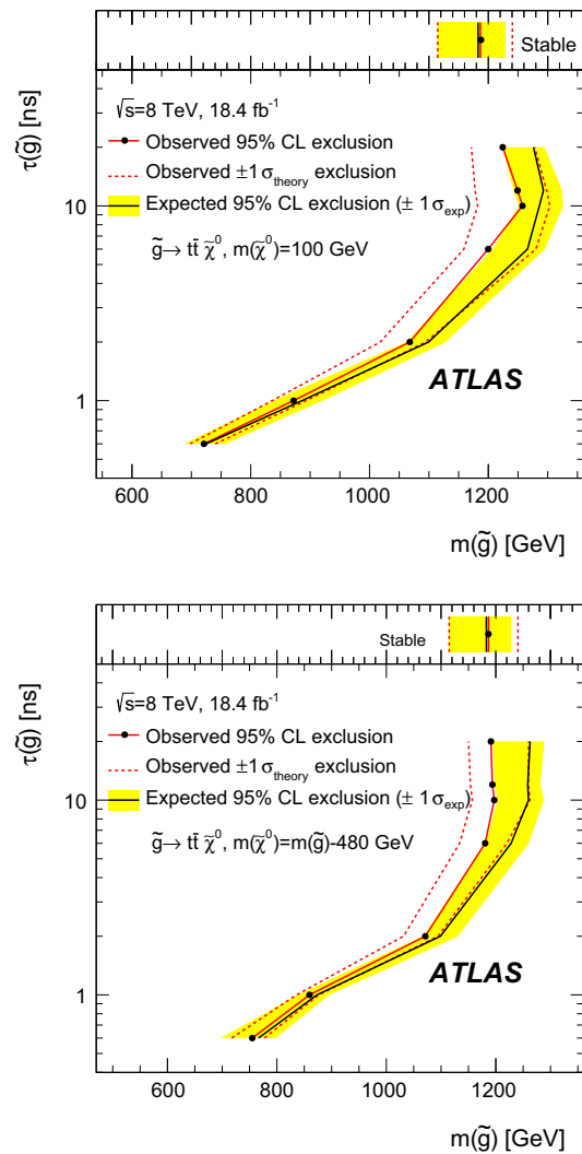
Fig. 9 The excluded range of lifetimes as a function of gluino mass for gluino R -hadrons decaying into t\bar{t} plus a light neutralino of mass m(\tilde{\chi}_1^0) = 100\text{ GeV} (top) or a heavy neutralino of mass m(\tilde{\chi}_1^0) = m(\tilde{g}) - 480\text{ GeV} (bottom). The expected exclusion, with its experimental \pm 1\sigma band, is given with respect to the nominal theoretical cross section
