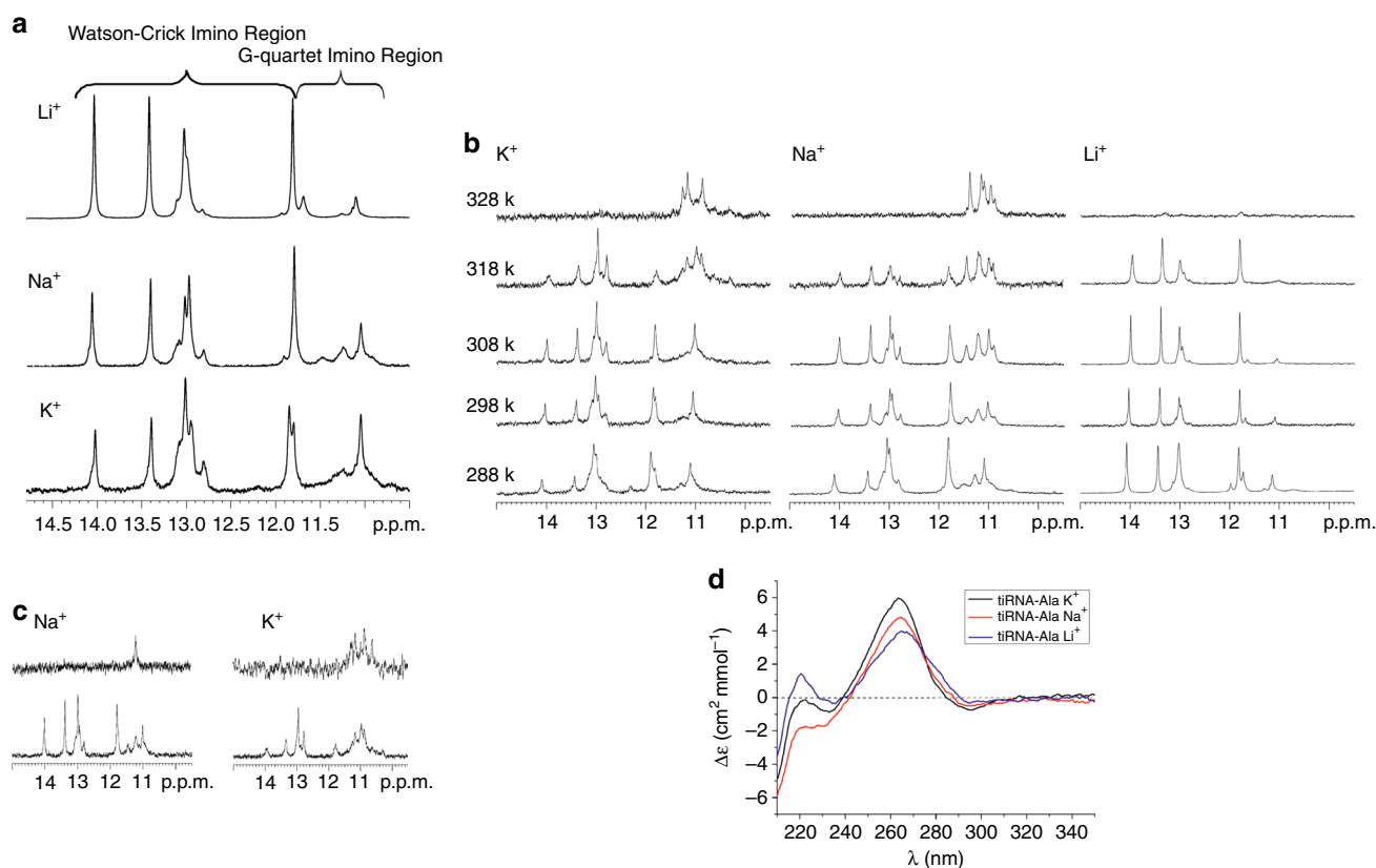
Fig. 2 NMR spectra confirm G-quadruplex formation. a Imino region of the ^1H NMR spectra of 5'tiRNA Ala . Spectra were recorded at 25 °C in 90% H_2O/10\% D_2O (v/v) in the presence of 50 mM KCl, 10 mM potassium phosphate, 0.1 mM EDTA, pH 6.8 (top panel), 150 mM NaCl, 10 mM sodium phosphate, 0.1 mM EDTA, pH 6.8 (middle panel), and 150 mM LiCl, 10 mM Tris-HCl, 0.1 mM EDTA, pH 6.8 (bottom panel). b Temperature dependence of the imino region of the ^1H NMR spectra of 5'tiRNA Ala . Spectra were recorded in 90% H_2O/10\% D_2O (v/v) in the presence of 50 mM KCl, 10 mM potassium phosphate, 0.1 mM EDTA, pH 6.8 (left panels), 150 mM NaCl, 10 mM sodium phosphate, 0.1 mM EDTA, pH 6.8 (middle panels), and 150 mM LiCl, 10 mM Tris-HCl, 0.1 mM EDTA, pH 6.8 (right panels). c Imino region of 5'tiRNA Ala in 90% H_2O/10\% D_2O (lower panels) and after 12 h in D_2O (upper panels) at 45 °C in the presence of 150 mM NaCl, 10 mM sodium phosphate, 0.1 mM EDTA, pH 6.8 (left panels) and 50 mM KCl, 10 mM potassium phosphate and 0.1 mM EDTA, pH 6.8 (right panels). d CD spectra of 5'tiRNA Ala at 25 °C. The spectra were recorded in the presence of 50 mM KCl, 10 mM potassium phosphate and 0.1 mM EDTA, pH 6.8 (black), 150 mM NaCl, 10 mM sodium phosphate, 0.1 mM EDTA, pH 6.8 (red) and 150 mM LiCl, 10 mM Tris-HCl, 0.1 mM EDTA, pH 6.8 (blue)
