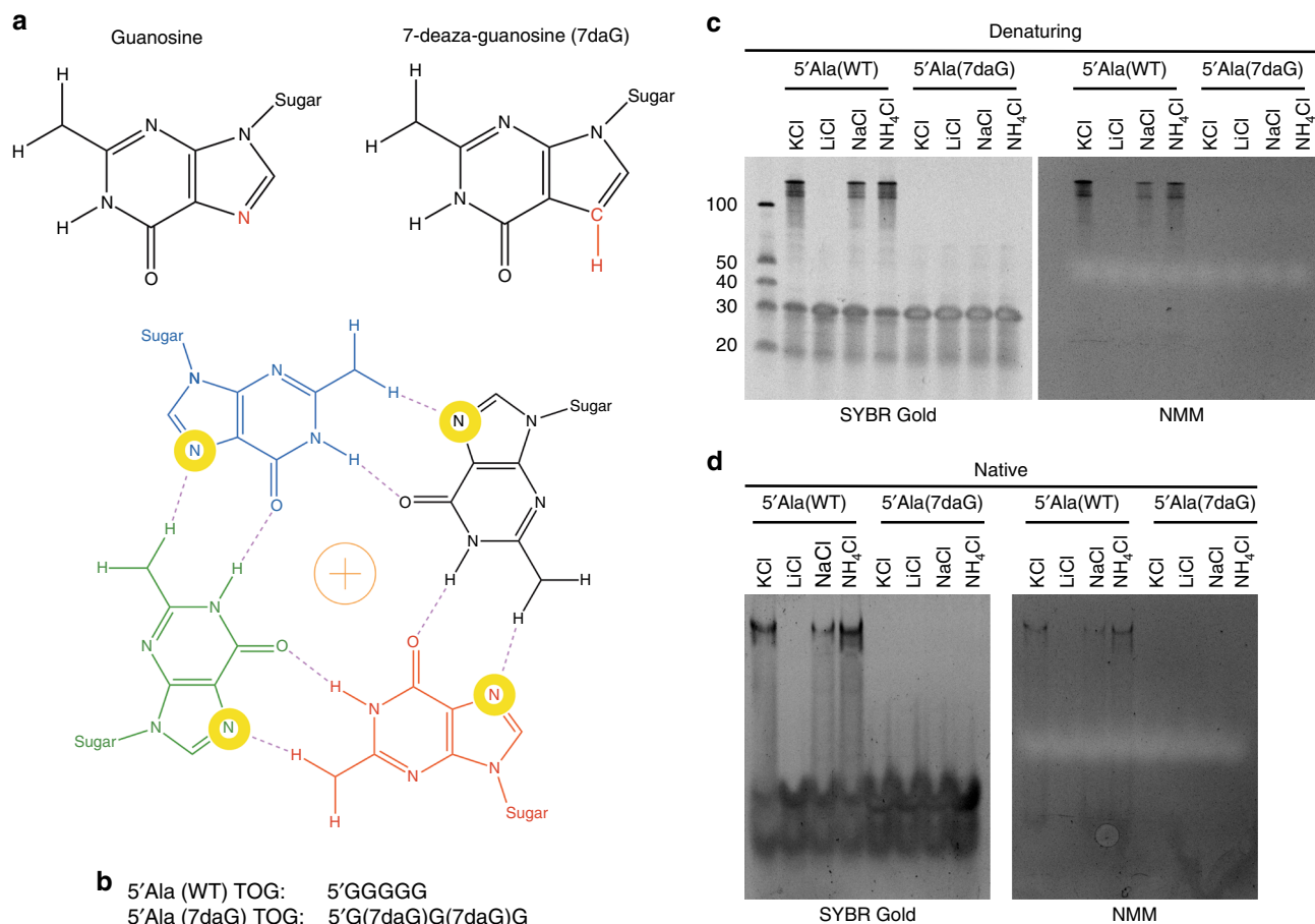
Fig. 4 Substitution of guanines in 5'TOG motif with 7-deazaguanine prevents RG4 formation. a 7-deazaguanine derivative replaces the azide group at position 7 with a methine group (highlighted). Interaction with the hydrogen of the methine group is essential for Hoogsteen basepairing in a G-quartet. b Guanines at position 2 and 4 in the 5'TOG motif of 5'tiRNA Ala were substituted with 7-deazaguanine ( c , d ) 5'tiRNA Ala (WT) or 5'tiRNA Ala (7daG) were equilibrated overnight in indicated salt solution and analyzed on denaturing c or native d gel and post-stained with SYBR gold (left panels) to detect total RNA or NMM (right panels) to detect RG4 structures. Regardless of ionic condition, 5'tiRNA Ala (7daG) failed to form RG4 structure highlighting the importance of Hoogsteen base pairing for RG4 formation
