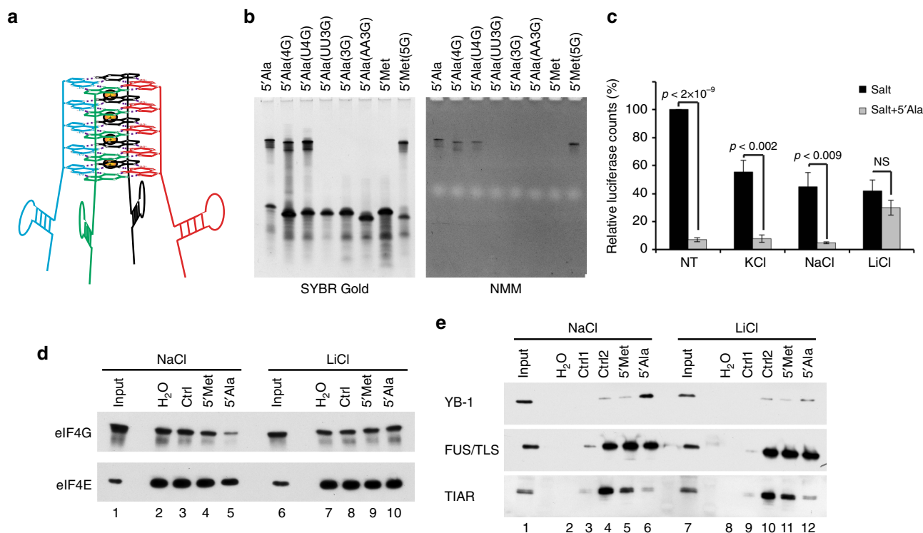
Fig. 3 Deletion of RG4 structures in 5'tiRNA Ala through ionic equilibration abolishes activity. a Model of tetrameric 5'tiRNA Ala coordinated by a central G-quadruplex core containing 5 stacked G-quartets. b The 5'TOG motif of 5'tiRNA Ala was mutated to varying extents. Indicated 5'tiRNA Ala mutants were run on a 15% denaturing acrylamide gel and post-stained with SYBR gold or NMM to detect total RNA or RG4, respectively. The propensity to form RG4 structures correlated with the bioactivity of each tiRNA (Supplementary Table 2). c 5'tiRNA Ala was equilibrated overnight in indicated salt or left untreated (NT). In vitro translation assays were carried out in rabbit reticulocyte lysate using polyadenylated NanoLuc RNA as a reporter. To each, 1 μl of 100 pmol salt equilibrated 5'tiRNA Ala or 1 μl of indicated salt was added prior to initiating translation reaction. Depletion of RG4 structure of 5'tiRNA Ala through equilibration in Li + ions abolished the ability of 5'tiRNA Ala to repress translation. d eIF4F was assembled onto m 7 GTP agarose and challenged with indicated RNAs equilibrated in NaCl or LiCl. Depletion of RG4 structures through equilibration in Li + ions abrogated the ability of the tiRNA to displace eIF4G or eIF4E from m 7 GTP cap. e RNPs were purified from U2OS lysates using biotinylated RNAs equilibrated in indicated salt solutions. Depletion of RG4 structures reduced 5'tiRNA Ala 's association with YB-1, a key regulator of 5'tiRNA Ala induced stress granules, to background levels. The interaction of 5'tiRNA Ala with FUS/TLS or TIAR was unaltered through ionic equilibration.
