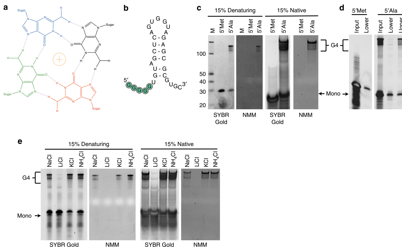
Fig. 1 5TOG containing tiRNAs exist in two distinct and interconvertible forms. a G-quartet formation by guanines. b Predicted secondary structure of 5'tiRNA Ala with a predominant hairpin structure. 5'TOG motif is indicated in green. c Indicated RNAs were ran on a 15% acrylamide denaturing gel (left panels) or native gel (right panels). Gels were post-stained with either SYBR gold to detect total RNA or NMM to detect RG4 structures. 5'tiRNA Ala ran at the expected 31 nts, but also at ~120 nts. Only the more slowly running band stained with NMM, indicating it contained RG4s. This more slowly migrating band persisted under denaturing conditions. d Indicated 5'tiRNAs were ran on a 15% denaturing acrylamide gel and either upper or lower species were gel purified and reanalysed on a denaturing acrylamide gel and post-stained with SYBR gold. A portion of the lower band re-equilibrated to the upper band and vice-a-versa. e 5'tiRNA Ala was equilibrated overnight in 100 mM of indicated salts. RNAs were analyzed on denaturing (left panels) or native gels (right panels) and post-stained with SYBR gold or NMM. Results demonstrate that NMM staining, more slowly migrating band disassembles in the presence of Li + ions
