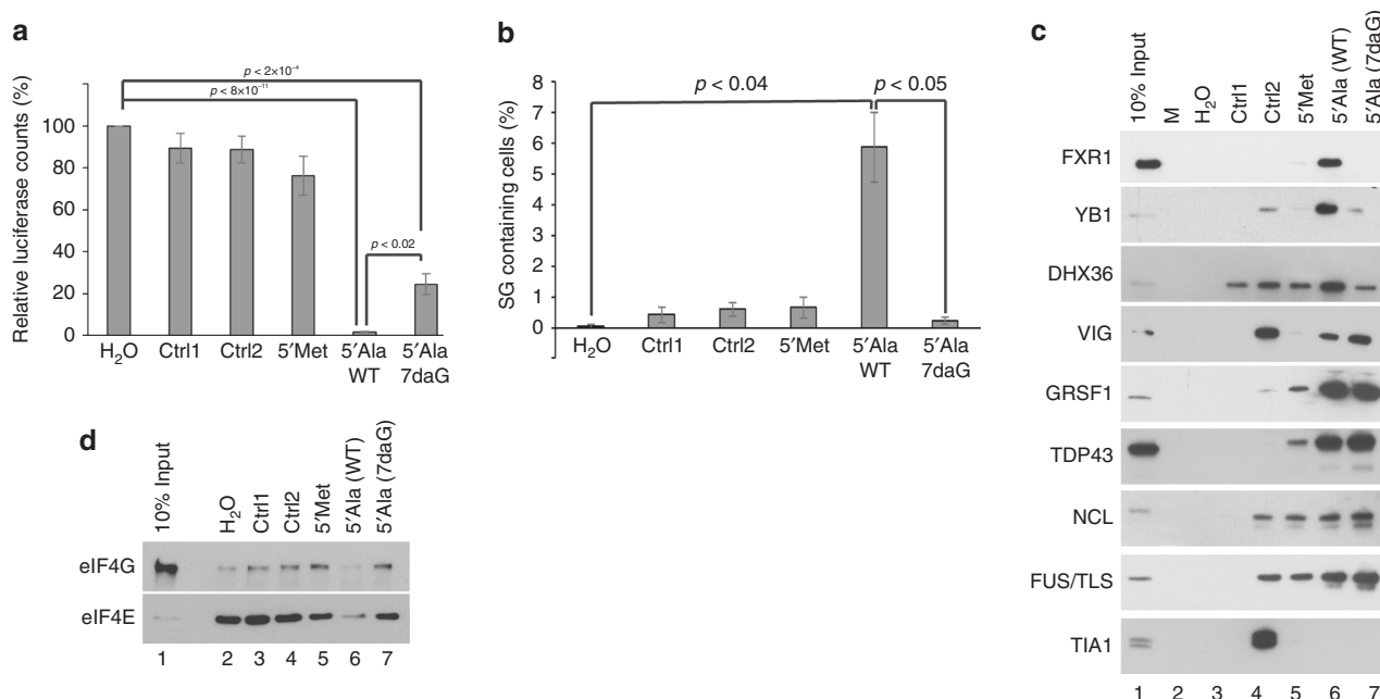
Fig. 5 7-deazaguanine substitutions in 5'tiRNA Ala prevent bioactivity. a In vitro translation assay in rabbit reticulocyte lysate using NanoLuc reporter to monitor translation efficiency. Substitution of two guanines in 5'tiRNA Ala reduces its ability to repress translation. b Indicated RNAs were transfected into U2OS cells and stress granule formation was monitored through immunofluorescence. 5'tiRNA Ala (WT) readily induces the formation of SGs, while 5'tiRNA Ala (7daG) fails to. c RNA affinity purifications using indicated RNAs from U2OS lysates. Loss of RG4 forming ability in 5'tiRNA Ala (7daG) correlates with loss of binding to YB-1, a protein required for tiRNA mediated SG formation. 5'tiRNA Ala (7daG) also loses the ability to bind to Fxr1 and DHX36, previously identified RG4 binding proteins. In contrast, Vigilin, GRSF1, and TDP43 bind 5'tiRNA Ala regardless of its ability to form RG4. d Inhibition of RG4 formation in 5'tiRNA Ala through incorporation of 7-deazaguanine abrogates its ability to displace eIF4F from m 7 GTP agarose
