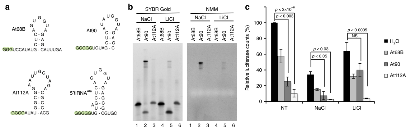
Fig. 6 tRNA fragments from Arabidopsis thaliana form RG4 which are required for their activity. a Secondary structures of three 5'tiRNA species previously identified in salt stressed A. thaliana harboring putative 5TOG motifs. b Analysis of A. thaliana tiRNAs on 15% denaturing acrylamide gel post-stained with either SYBR Gold or NMM to detect total RNA or RG4 structures, respectively. AtRNA90 forms a strong RG4 positive band which runs in a similar manner to 5'tiRNA Ala . Upon equilibration in LiCl, the more slowly migrating RG4 positive band disappears. c In vitro translation in rabbit reticulocyte lysates using salt equilibrated or untreated (NT) A. thaliana RNAs. Depletion of RG4 structures in AtRNA90 inhibits its ability to repress translation. However, other active A. thaliana tiRNAs repress translations despite ionic equilibration suggesting they inhibit translation via an alternative mechanism
