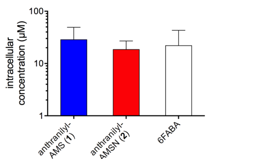
Figure 4. Compound accumulation in P. aeruginosa strain PA14 after incubation with 1000 \mu\text{M} extracellular concentration for 30 min.
