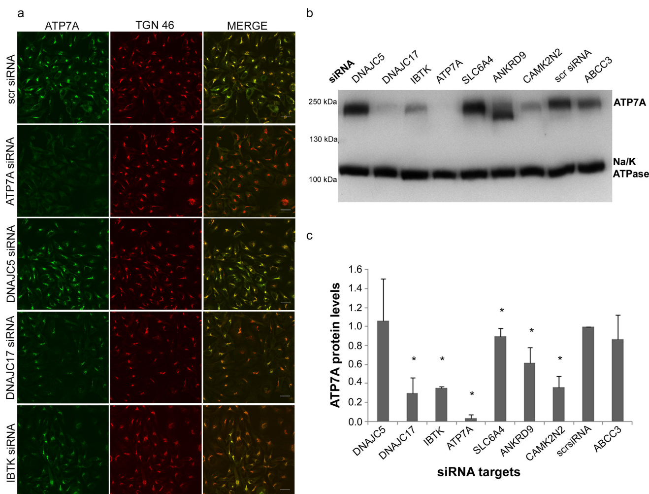
Figure 4. Characterization of targets that affect copper levels in HeLa cells
