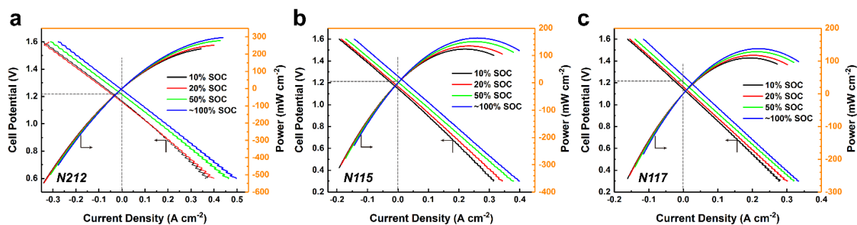
Figure. 6 Electrochemical performance of a DHBQ/ \text{K}_4\text{Fe}(\text{CN})_6 cell. Electrolytes comprise 6 mL of 0.5 M DHBQ in 2M KOH (the negolyte) and 22.5 mL of 0.4 M potassium ferrocyanide ( \text{K}_4\text{Fe}(\text{CN})_6 ) in 1M KOH (the posolyte). The cell-polarization plots, composed of cell potential (left vertical) and power density (right vertical) versus discharge current density, correspond to the cell assembled with (a) Nafion 212 membrane (N212), (b) Nafion 115 membrane (N115) and (c) Nafion 117 membrane (N117). The dashed lines indicate open circuit potential at 50% SOC.
