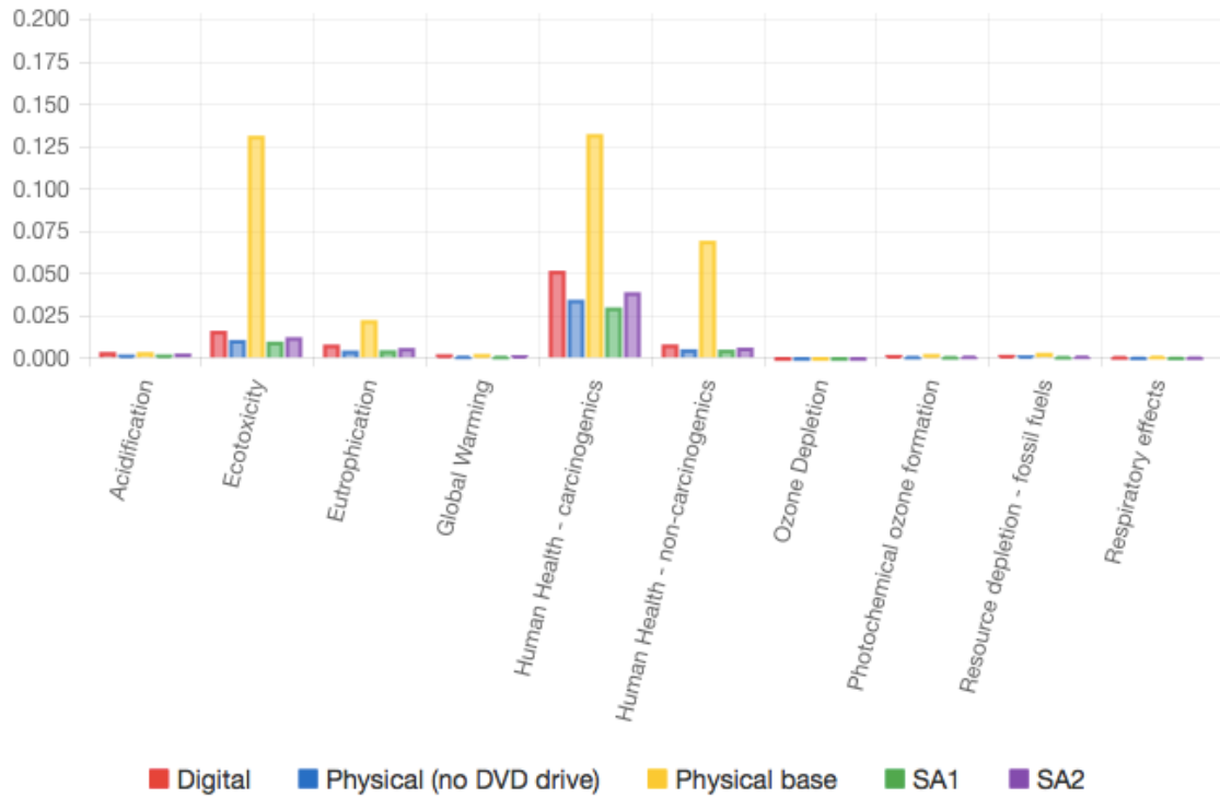
Figure 11. Normalized bar chart for PC, base cases and digital sensitivity analyses (from OpenLCA).
