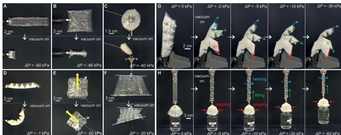
Fig. 3. Various basic actuation motions and programmable pseudosequential actuation with multiple degrees of freedom. (A) A 19 cm-long linear zigzag actuator contracts to a compressed structure shorter than 2 cm. The 1D contraction ratio is \sim 90\% . (B) A 2D origami skeleton using the Miura-ori patterns (area: 11 \times 10 cm 2 ) can contract to a dense bar-shaped structure (area: 9 \times 1 cm 2 ). The 2D area contraction ratio approaches 92%. (C) A 3D “magic-ball” origami using the water-bomb pattern (radius: 3.5 cm) contracts to a compacted cylindrical structure (radius: 0.9 cm; height: 6.5 cm). The 3D volume decreases 91% after this contraction. (D) Bending motion can be achieved by using an asymmetrical beam structure as the skeleton. (E) Using a flasher origami pattern as the skeleton, the actuator rotates more than 90 degrees around its center, and its 2D surface contracts by 54% simultaneously. (F) A complex out-of-plane motion combining torsion and contraction can be programmed through a 2D Miura-ori origami pattern with select folds weakened. (G) Three fingers on a robotic hand are actuated at different rates using a single control of the internal air pressure. The skeletal structure of this robotic hand is 3D printed from nylon. Different hinge strengths inside the structural voids are designed for these three fingers, which produce significantly different bending stiffnesses: k_{s1} (red) < k_{s2} (green) < k_{s3} (blue). The bending stiffness of each finger determines its own bending angle at a certain internal pressure level. (H) A bottle of water is gripped, lifted, and twisted by a single-channel vacuum-driven robotic arm. The robotic arm has a modular structure including a cup-shaped gripper and a cylindrical lifter. The gripper uses a polyester magic-ball origami as its skeleton, while a much stiffer compression spring (302 stainless steel) is used as the lifter’s skeleton. When the internal pressure decreases smoothly, the gripping motion will always start first, then the lifting and twisting motions start later as the internal pressure reduces further.
