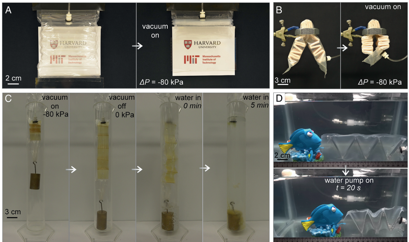
Fig. 2. Linear zigzag actuators made of a variety of materials using different fabrication methods. (A) A transparent actuator lifts a clear acrylic plate. Skeleton material ( SkeM ): 0.254 mm transparent polyester sheet. Fabrication method ( FM ): laser cutting and manual folding. Skin material ( SkiM ): 0.102 mm transparent PVC film (Vinyl). Driving fluid ( DF ): air. (B) A soft linear actuator contracts well even when it is confined into a metal screw nut. SkeM : silicone rubber (M4601). FM : casting. SkiM : 0.24 mm TPU film. DF : air. (C) A vacuum-driven water-soluble actuator is dissolved in hot water ( \approx 70^\circ\text{C} ) within 5 min. SkeM : polyvinyl alcohol (PVA). FM : 3D printing. SkiM : 0.025 mm PVA film. DF : air. (D) A water pump-driven hydraulic actuator pulls an underwater object for 3.5 cm in 20 s. SkeM : 0.254 mm stainless steel (316). FM : manual forming. SkiM : 0.24 mm TPU film. DF : water.
