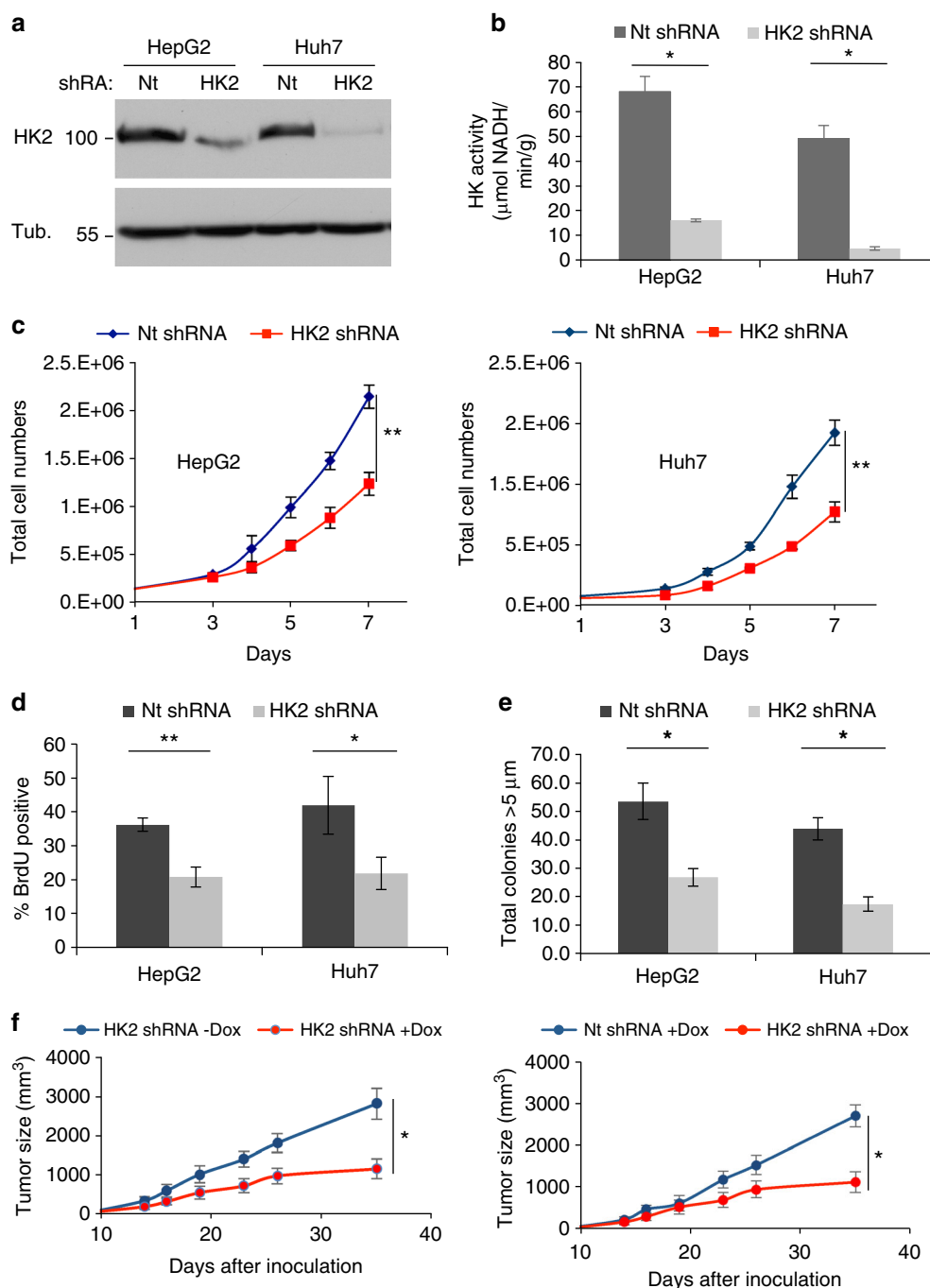
Fig. 2 Effect of HK2 knockdown on tumorigenicity of human HCC cells. a Immunoblot analysis of inducible HK2 KD in HepG2 and Huh7 cells. b In vitro hexokinase activity assays upon inducible HK2 KD. c Cell proliferation curves. d BrdU incorporation analysis. Bar graphs show the percentage of BrdU-positive cells. e Anchorage-independent growth on soft agar. The cells were exposed to Dox for 3 days prior to analysis and maintained in Dox throughout the analyses. Bar graphs show the number of colonies larger than 5 \mu\text{m} . f In vivo tumor growth. Cells were inoculated into mice; after tumor detection, mice were fed either regular chow diet or with a Dox-infused diet. The left panel shows tumor growth of the Huh7 cells with inducible HK KD in either the absence or presence of Dox, and the right panel shows the tumor growth of the inducible HK KD in the presence of Dox compared to tumor growth of control cells in the presence of Dox ( n = 6 ). Nt and HK2 shRNA indicate Dox-inducible non-targeting and HK2 shRNA, respectively. See Methods for experimental details. The results represent mean \pm SEM, * p < 0.05 , ** p < 0.01 , by Student's t -test
