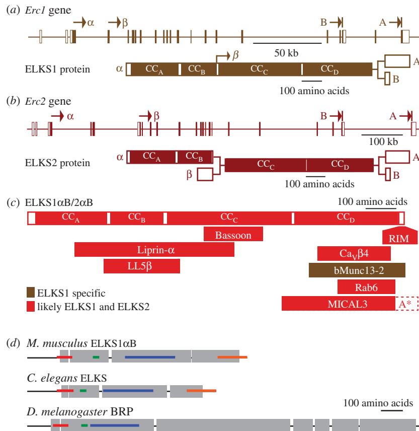
Figure 2. ELKS genes and proteins. (a) Erc1 mouse gene structure (top) and ELKS1 protein structure arising from multiple start codons ( \alpha - and \beta -isoforms) or C-terminal splice variants (A- and B-isoforms). White boxes in the Erc1 gene indicate untranslated regions (UTR), filled boxes are protein coding regions (modelled after Liu et al. [57]). (b) Erc2 mouse gene structure (top) and ELKS2 protein structure arising from alternatively spliced N-terminal exons ( \alpha - and \beta -isoforms, respectively) or C-terminal splice variants (A- and B-isoforms). White boxes in the Erc2 gene indicate untranslated regions (UTR), shaded boxes are protein coding regions (modelled after Kaeser et al. [56]). (c) ELKS protein interaction map exemplified by the prototypic \alpha B-isoform. A*, the MICAL3 binding site may extend into the A-variant specific C-terminus. (d) Coiled-coil structure prediction (grey boxes) of Mus musculus (XP_017176819), C. elegans (NP_500329) and Drosophila melanogaster (NP_001036535) ELKS1 \alpha B/ELKS/BRP using MARCOIL [74]. Coloured bars indicate regions with greater than 25% amino acid sequence identity between species. Red, M.m. — 163 REND-RKDE 204 , C.e. — 157 REYE-RRDE 198 , D.m. — 123 RELG-RKEE 164 ; green, M.m. — 303 NARD-QSKG 320 , C.e. — 233 LRER-ESGS 251 , D.m. — 247 IARD-QAKG 264 ; blue, M.m. — 436 MKNK-QGDL 668 , C.e. — 340 MRMK-QKEL 543 , D.m. — 280 MAQK-ESEV 485 ; orange, M.m. — 875 ERRK-GIWA 976 , C.e. — 720 ERRQ-GIWA 836 (modelled after Wagh et al. [71]).
