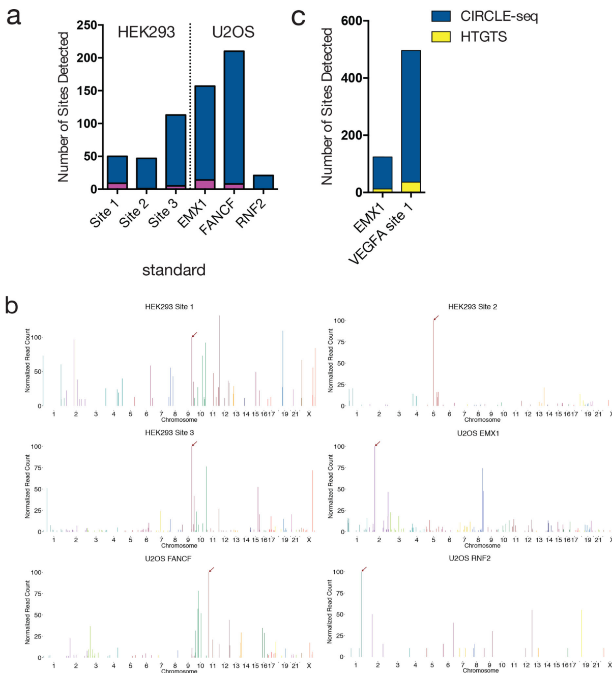
Figure 2. Comparisons of CIRCLE-seq with cell-based GUIDE-seq and HTGTS methods
