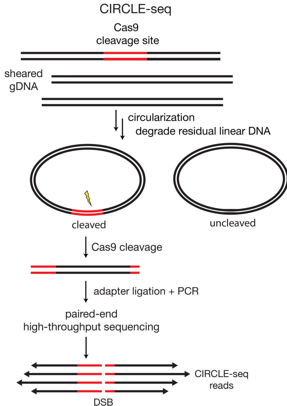
Figure 1. Overview of CIRCLE-seq methods for detection of genome-wide CRISPR-Cas9 nuclease cleavage
