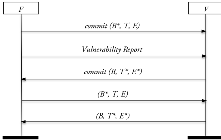
FIGURE 1: THE SVC PROTOCOL
