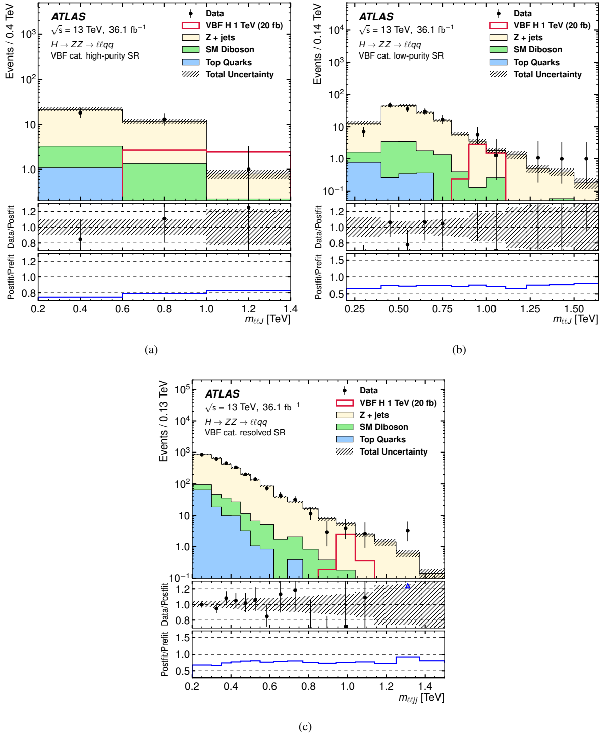
Figure 7: Comparisons of the observed data and expected background distributions of the final discriminants of the VBF category for the H \rightarrow ZZ \rightarrow \ell\ell q\bar{q} search: m_{\ell\ell j\bar{j}} of (a) high-purity and (b) low-purity signal regions; (c) m_{\ell\ell j\bar{j}} of the resolved signal region. For illustration, expected distributions from the VBF production of a 1 TeV Higgs boson with \sigma \times \mathcal{B}(H \rightarrow ZZ) = 20 fb are also shown. The middle panes show the ratios of the observed data to the background predictions. The uncertainty in the total background prediction, shown as bands, combines statistical and systematic contributions. The blue triangles in the middle panes indicate bins where the ratio is nonzero and outside the vertical range of the plot. The bottom panes show the ratios of the post-fit and pre-fit background predictions.
