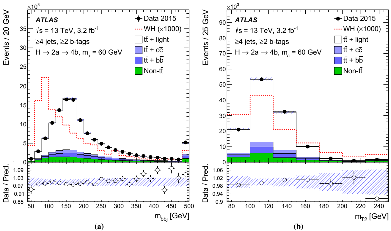
Fig. 3 Comparison of data with the SM background predictions for the distributions of a m_{bbj} and b m_{T2} in the sample that is inclusive in number of jets and b -tagged jets. Distributions for the signal model ( WH, H \rightarrow 2a \rightarrow 4b ), with m_a = 60 GeV, normalised to the SM
