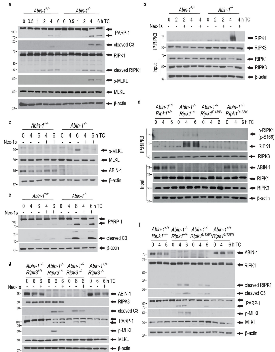
Figure 4. Inhibition of necroptosis prolongs cell survival but has no effect on caspase activation in Abin-1 -/- cells treated with TNFα/CHX
