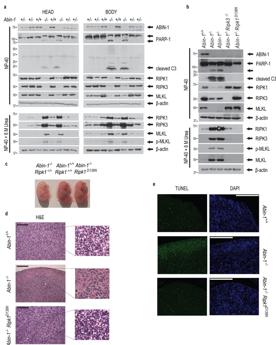
Figure 7. The presence of hallmarks of both apoptosis and necroptosis in Abin-1 -/- embryos (E16.5)
