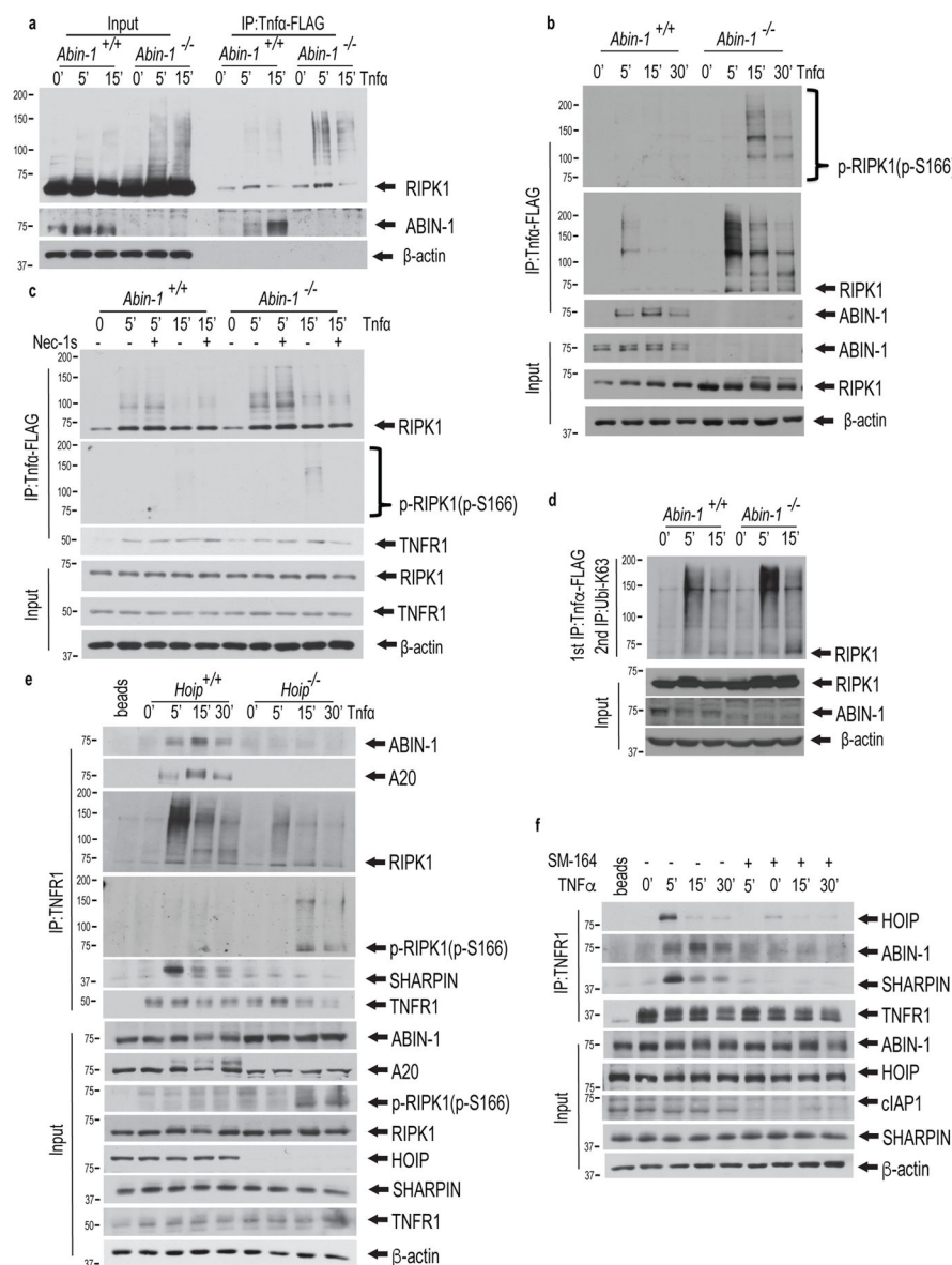
Figure 5. Increased K63 ubiquitination of RIPK1 in Abin-1 -/- MEFs stimulated by TNFα (a–c) WT ( Abin-1 +/+ ) and Abin-1 -/- MEFs were stimulated by Flag-TNFα (100 ng/ml) for indicated periods of time and (c) Nec-1s was added in selected samples as indicated. TNF-RSC (Complex I) was immunoprecipitated using anti-FLAG resin and the recruitment of ABIN-1 and RIPK1 was analyzed by western blotting using indicated antibodies (a). The activation of RIPK1 was analyzed by western blotting using anti-p-RIPK1(p-S166) ab (b–c). TNFR1 was a control for TNF-RSC (c). β-actin is a loading control. (d) WT ( Abin-1 +/+ ) and Abin-1 -/- MEFs were stimulated by Flag-TNFα (100 ng/ml) for indicated periods of time and the cell lysates were immunoprecipitated using anti-FLAG resin. The immunocomplexes were then denatured in 6M urea. K63-chain specific ubiquitin antibody was used in the second immunoprecipitation in 3M urea to analyze RIPK1 ubiquitination in TNF-RSC by western blotting using anti-RIPK1. (e) Hoip +/+ and Hoip -/- MEFs were
