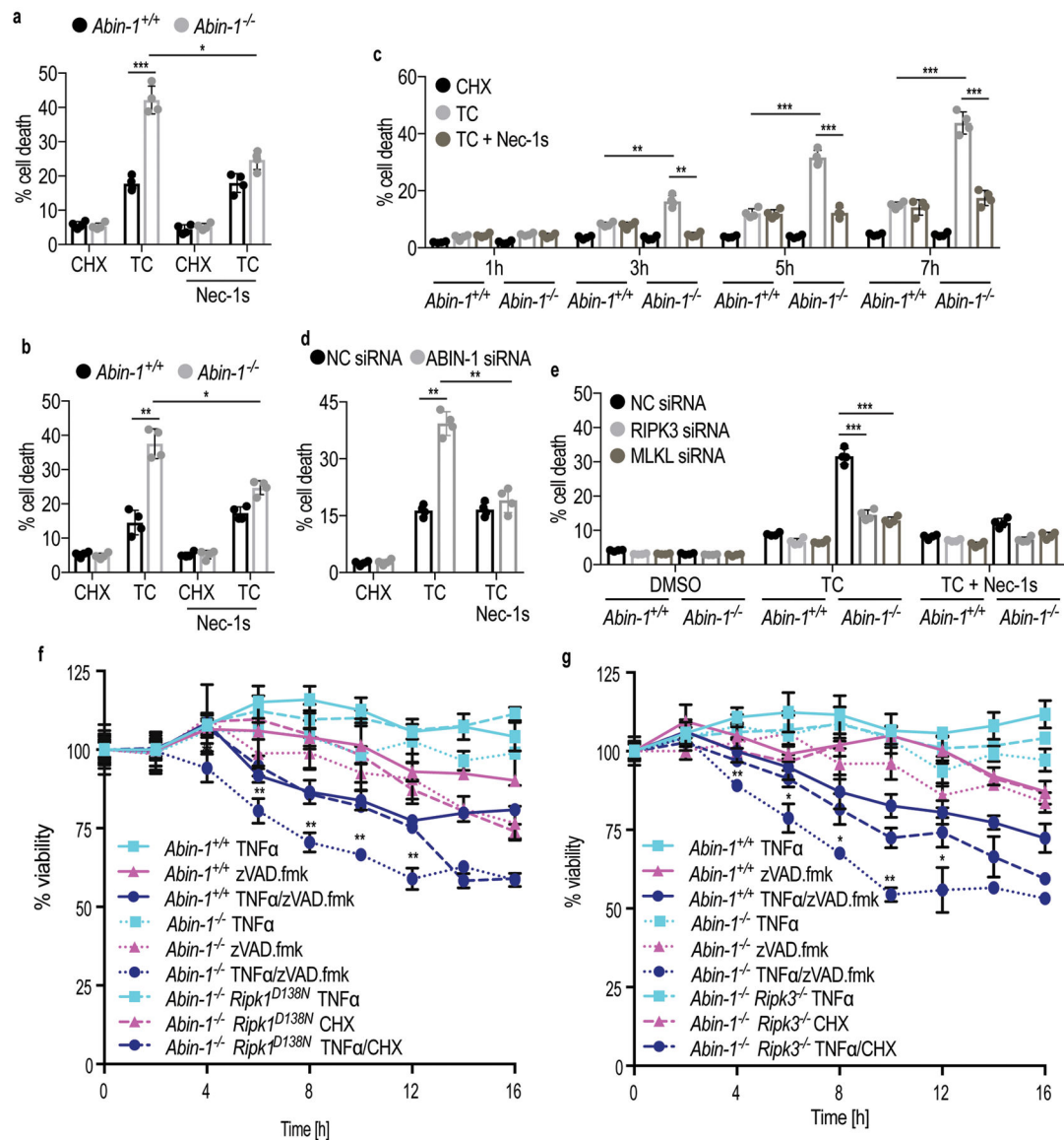
Figure 3. Inhibition of RIPK1, RIPK3 and MLKL prolongs the survival of apoptotic ABIN-1 deficient cells induced by TNFα/CHX
