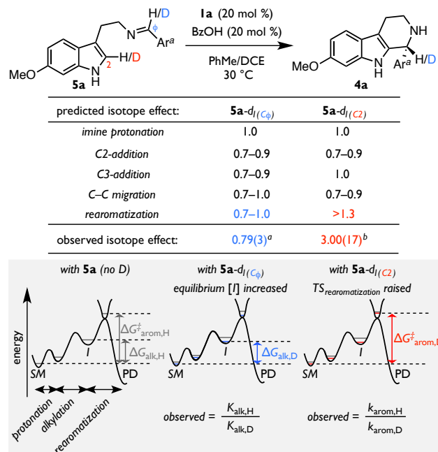
Figure 4. Isotope Effect Measurements. a Competition isotope effect determined from the ratio of recovered \mathbf{5a} and \mathbf{5a}\text{-}d_{1(\text{C}\Phi)} at low conversion. b Isotope effect determined from the relative first-order rate constants for formation of \mathbf{4a} measured independently with \mathbf{5a} and \mathbf{5a}\text{-}d_{1(\text{C}2)} . Rates are uncorrected for incomplete deuterium incorporation (94% D for \mathbf{5a}\text{-}d_{1(\text{C}2)} ). See ref 86. \text{Ar}^a = 4-cyanophenyl.
