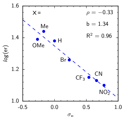
Figure 5. Co-Catalyst Structure–Reactivity–Enantioselectivity Relationships. Enantiomeric excess reported for the formation of 4b under the conditions shown. Relative rate constants ( k_{rel} ) determined from the first-order rate constants for formation of 4a under the conditions in Scheme 1. Ar^b = 4-chlorophenyl. Ar^F = 3,5-bis(trifluoromethyl)phenyl.
