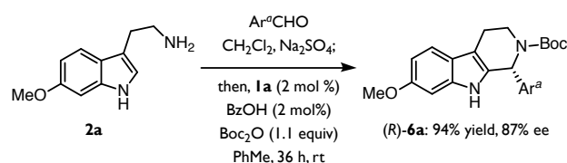
Figure 3. Kinetic Evidence for Product Inhibition and New Reaction Conditions for Minimizing Product Inhibition. See Scheme 1 for reaction conditions used for kinetic analysis; results from multiple independent runs are overlaid. \text{Ar}^a = 4-cyanophenyl. Boc = tert -butoxycarbonyl.
