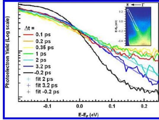
Figure 5.2 TrARPES on Bi 2 Te 3 studied by Hajlaoui et al. has focused on the thermalization process of the photoexcited electrons.
