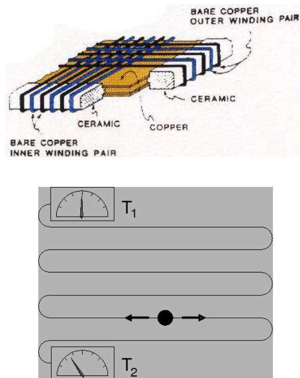
Figure 3.17 Schematics of delay-line detector. A delay-line detector is composed of two copper wires wound around a ceramic block perpendicular to each other into a mesh. When an electron pulse hits the detector, it generates two counter-propagating pulses along both wires. The time these pulses take to travel to the end of the wires are registered so that the position on the wire of the electron hit is known by the difference of the time.
