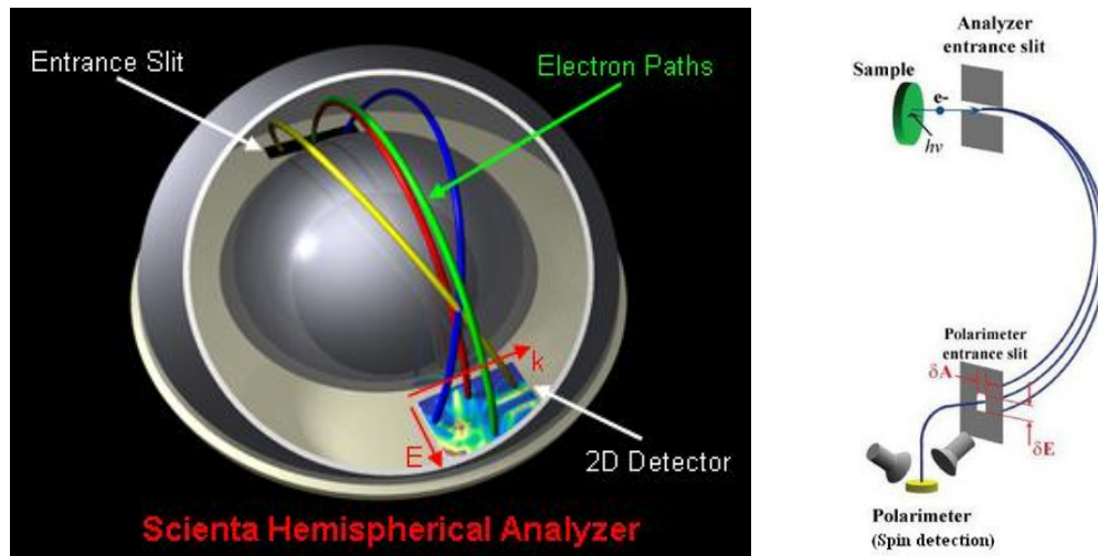
Figure 2.4 Left: A typical hemispherical electron energy analyzer. Electrons with different energies are separated by the voltage difference between the two hemispheres and the momenta of the electrons are mapped onto the other dimension of the 2D detector. Right panel shows a spin-resolved ARPES setup. Electrons with certain energy and momentum filtered by the hemispheres enter a hole and impinge on a gold foil with high energy. Electrons with different spins are scattered into different directions. Adapted from Z.-X. Shen lab website.
