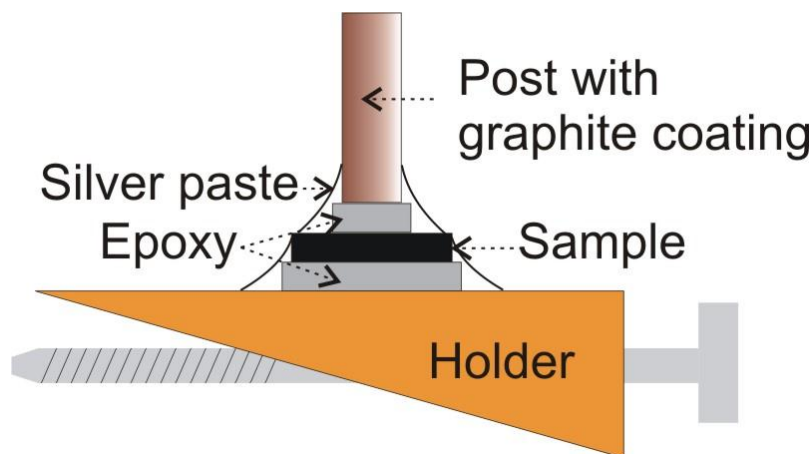
Figure 3.22 Sample prepared for cleaving. The sample is sandwiched in between the holder and the post by silver-epoxy. If the post is hit with mechanical force, it detaches with the top layer of the sample and exposes a fresh surface.
