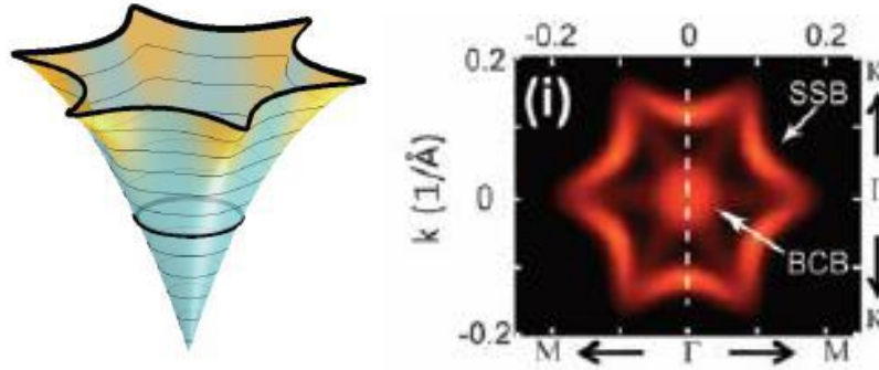
Figure 4.5 Hexagonal warping effect in \text{Bi}_2\text{Te}_3 . Left: constant energy contour of the hexagonally warped surface states from first principle calculation [4]. Right: constant energy cuts of the Fermi surface of \text{Bi}_2\text{Te}_3 . Adapted from [7].
