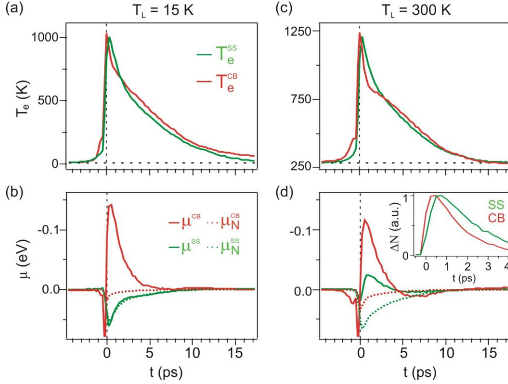
Figure 5.8 Electronic temperature and chemical potential dynamics for high doping sample. (a)
