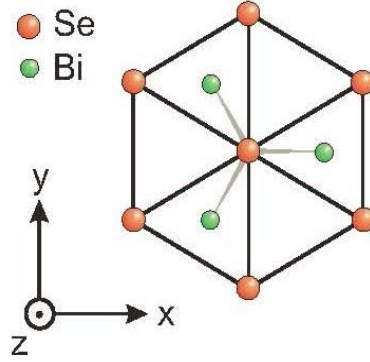
Figure 4.11 Trigonal crystal structure of \text{Bi}_2\text{Se}_3
