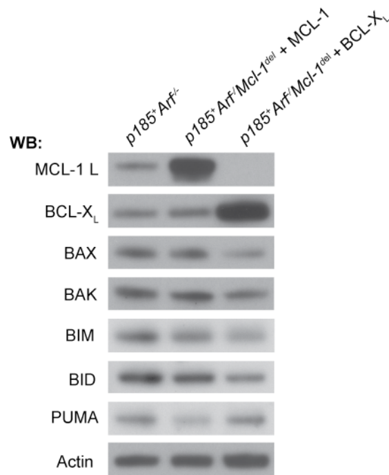
Figure 3.6 Western blot analysis of genetically-defined p185^{+} Arf^{-/-} B-ALL cells. Whereas the parental p185^{+} Arf^{-/-} B-ALL cells express both MCL-1 and BCL- X_L , MCL-1- and BCL- X_L -rescued p185^{+} Arf^{-/-} Mcl-1 -deleted B-ALL cells demonstrate overexpression of MCL-1 or BCL- X_L , respectively. Pro-apoptotic effectors, such as BAX, BAK, and BH3-only proteins, are expressed at relatively similar levels in all three cell lines.
