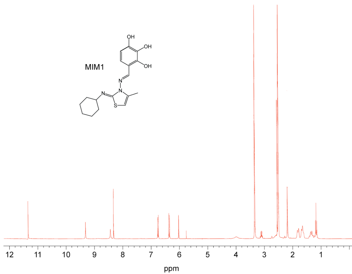
Figure 3.2. ^1\text{H} NMR spectrum of MIM1.
