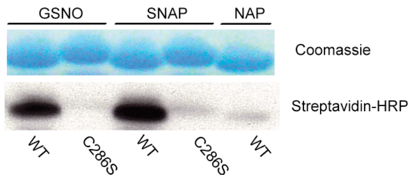
Figure 4.6. MCL-1ΔNΔC is S -nitrosylated in vitro . Wild-type MCL-1ΔNΔC, but not the C286S mutant, is nitrosylated by GSNO (40 μM) and SNAP (40 μM), but not by NAP (40 μM), as detected by the S-nitrosylated protein kit.
