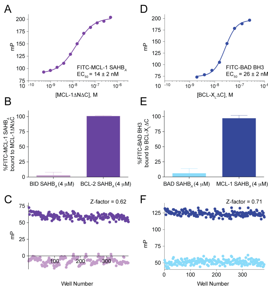
Figure 2.1. Development of a stapled peptide-based high-throughput competitive screening assay for identifying MCL-1-selective small molecules. (A-C) A high-throughput competitive FP binding assay was developed based on the direct binding interaction between FITC-MCL-1 SAHB A and MCL-1ΔNΔC (EC 50 , 14 nM), and validated for screening using a positive control for complete displacement (BID SAHB A ) and a negative control for no displacement (BCL-2 SAHB A ), yielding an assay Z-factor of 0.62. (D-F) To enrich for MCL-1-selective small molecules, a counter-screen was developed based on the direct binding interaction between FITC-BAD BH3 and BCL-X L ΔC (EC 50 , 26 nM), and validated for screening using a positive control for complete displacement (BAD SAHB A ) and a negative control for no displacement (MCL-1 SAHB A ), yielding an assay Z-factor of 0.71.
