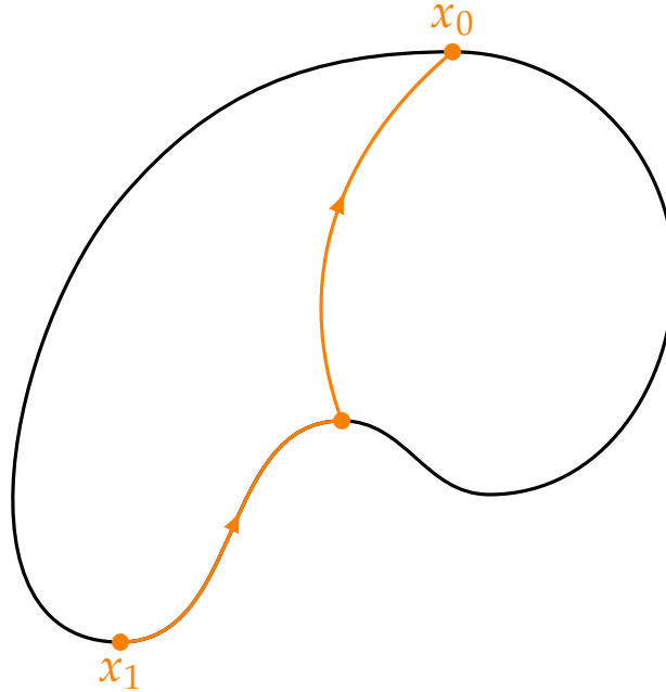
Figure 1.1: A breaking of a Morse gradient flow trajectory on the sphere at the boundary of the moduli space \mathcal{M}(x_0, x_1) \subset \overline{\mathcal{M}}(x_0, x_1) into a broken Morse trajectory through the point x_2 .
