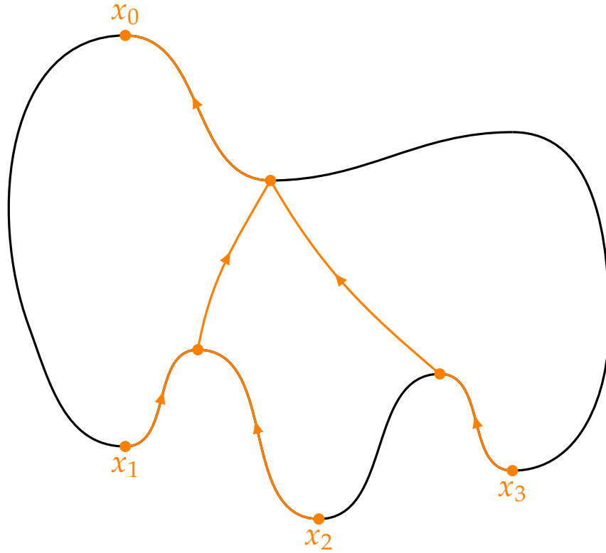
Figure 1.2: A Morse gradient flow tree with 3 inputs x_1 , x_2 , and x_3 , and output x_0 .
