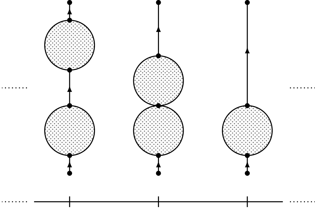
Figure 3.3: A schematic diagram depicting the nodal domain configuration lying at the common boundary point where two 1-dimensional strata of \overline{\mathcal{M}}_{\mathbf{p},n}(\mathbf{x})_1 are glued, this point obtained from domain configurations arising from a single application of the operation (2.2.b) or (2.2.c) respectively.
