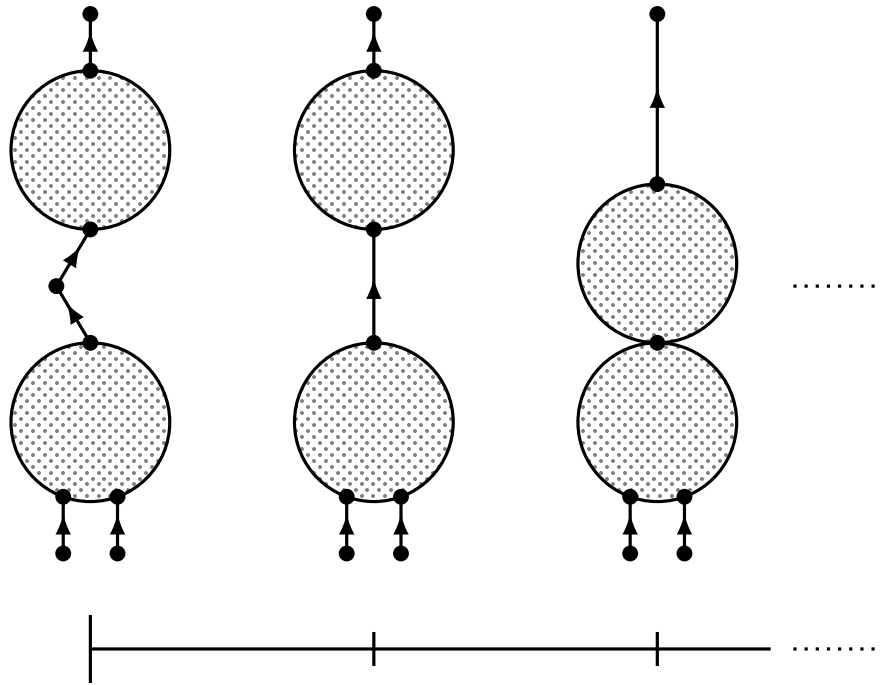
Figure 3.2: A representative diagram depicting a 1-parameter family meeting the boundary of the moduli space in which it resides.
