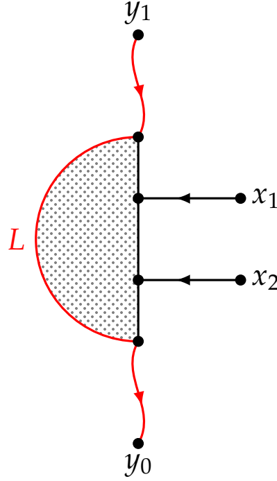
Figure 4.4: A schematic diagram of a pseudoholomorphic treed polygon obeying a spec (\mathbf{m}, \mathbf{x}, \beta) for a labeled type with module-shaped boundary labels \lambda^{L|2} , belonging to the moduli space \mathcal{M}_{\mathbf{p},3}(\lambda^{L|2}, \mathbf{x})_0 and therefore contributing to the module action map for \hat{C}(L) (c.f. Definition 4.22).
