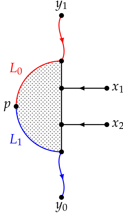
Figure 4.7: A schematic diagram of a pseudoholomorphic treed polygon obeying a spec (\mathbf{m}, \mathbf{x}, \beta) for a labeled type with morphism-shaped boundary labels \lambda^{(L_0, L_1)|^2} , belonging to the moduli space \mathcal{M}_{\mathbf{P}, 4}(\lambda^{(L_0, L_1)|^2}, \mathbf{x})_0 and therefore contributing to the morphism maps of the family Floer functor (c.f. Definition 4.26).
