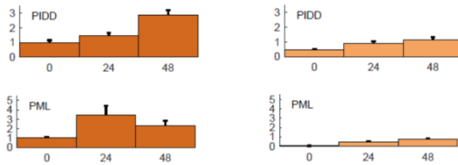
Figure 3.8: The expression profile of both PIDD and PML show increased expression in the long-term time frame of 24 and 48 hours (left panel). SiRNA against PIDD and PML suppress mRNA levels in response to irradiation (right panel).
