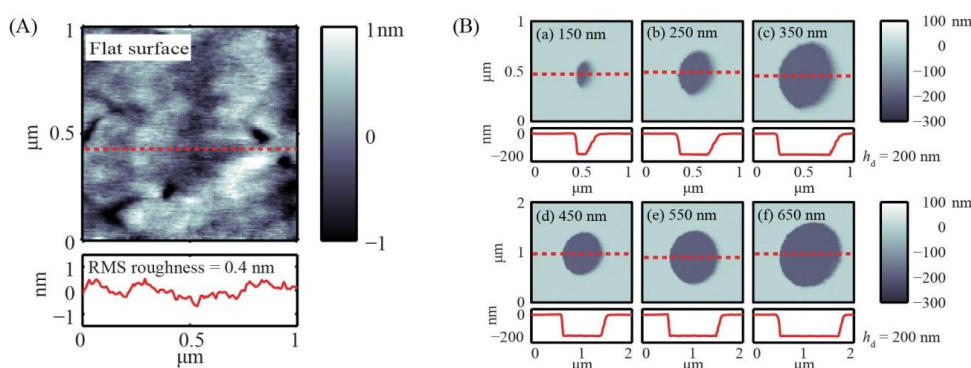
Figure 1.6 Atomic force microscope images of dimples
