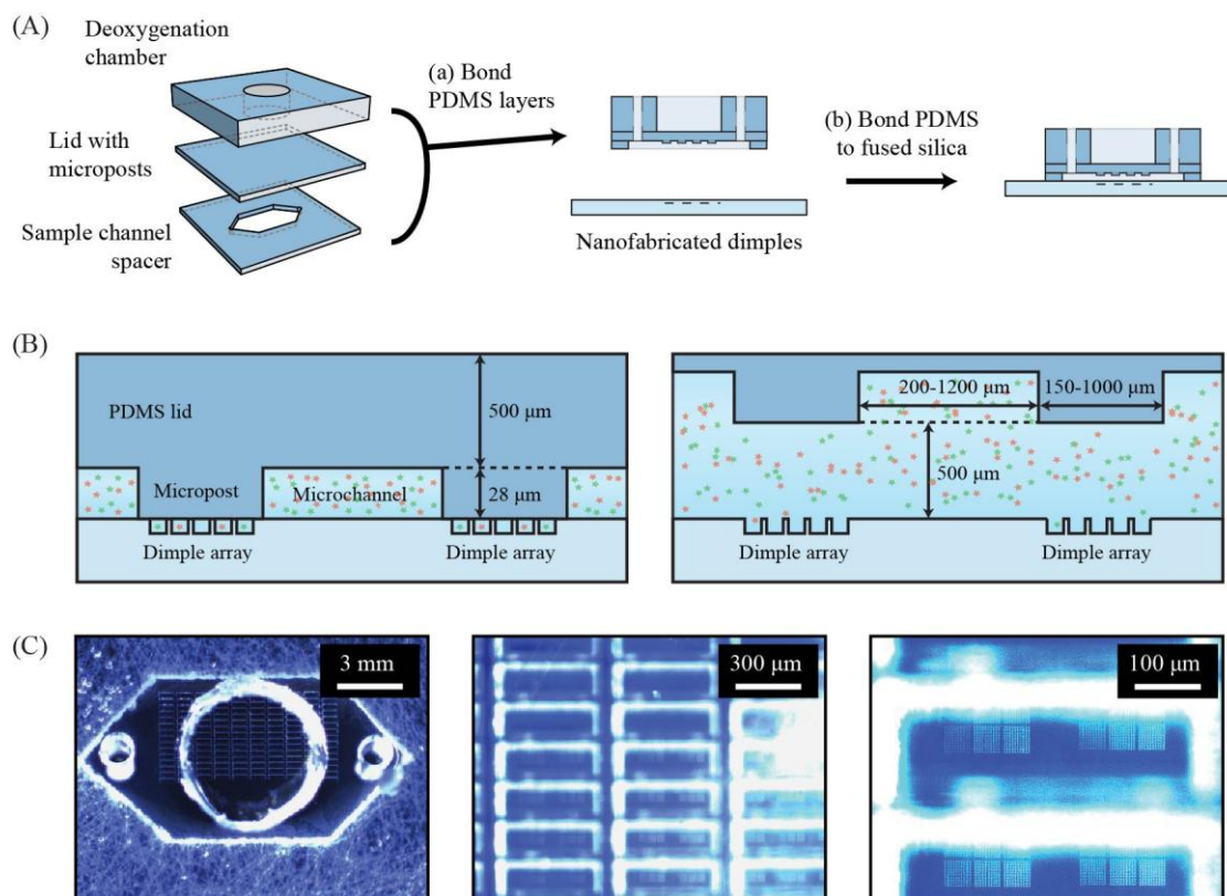
Figure 1.11 Lid-dimple assembly
