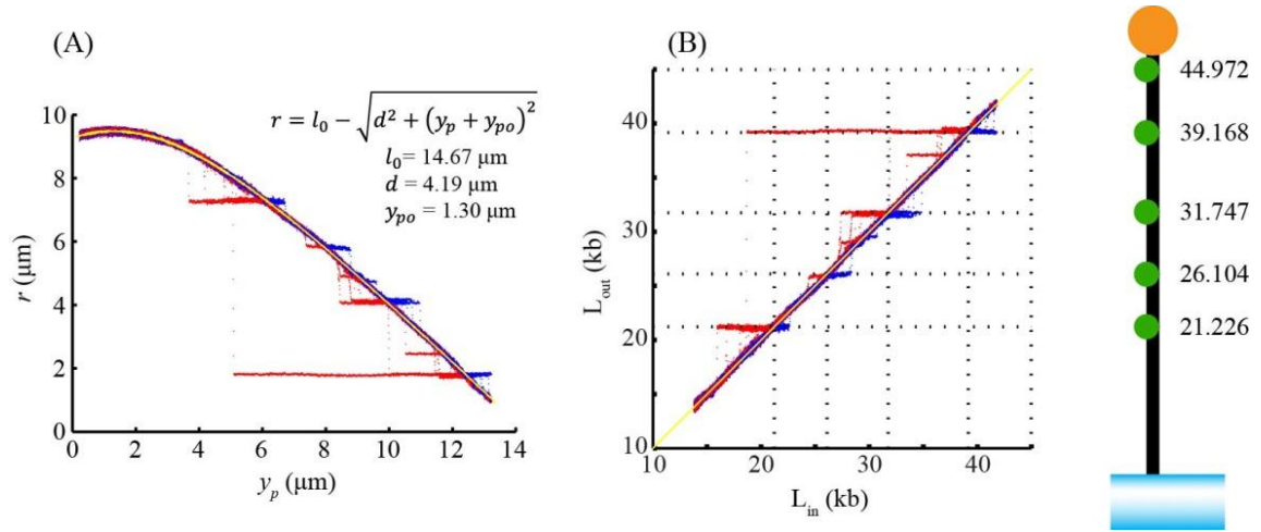
Figure 2.16 Mapping of EcoRI sites to sequences
