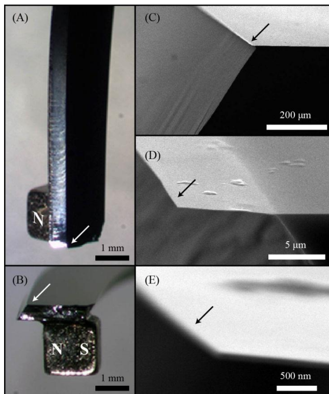
Figure 2.6 Images of silicon nitride knife
