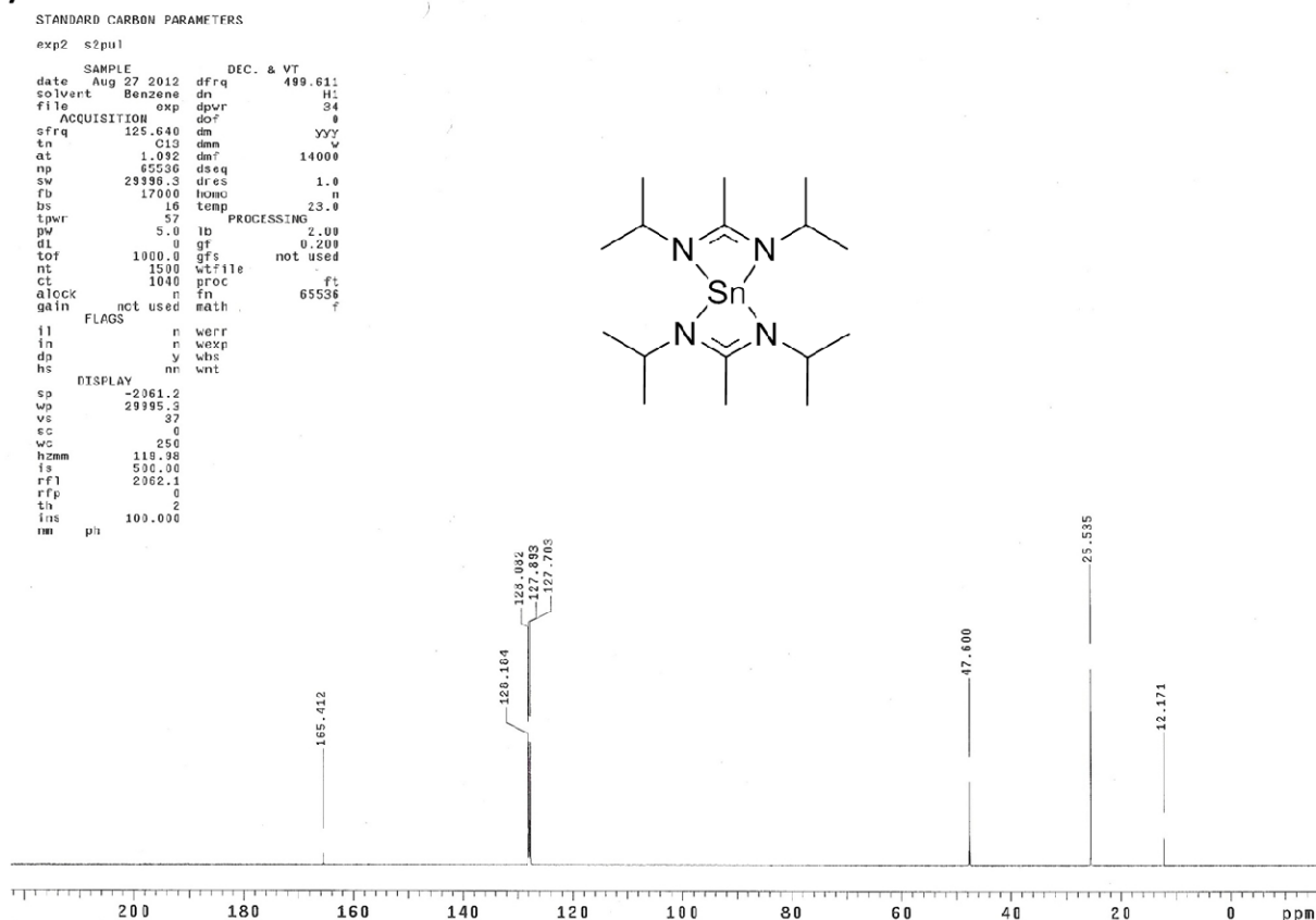
Figure A.3 (Continued): NMR Spectra (500MHz , \text{C}_6\text{D}_6 ) of bis(N,N'-diisopropylacetamido)tin(II): (c) ^{13}\text{C} NMR spectrum.
