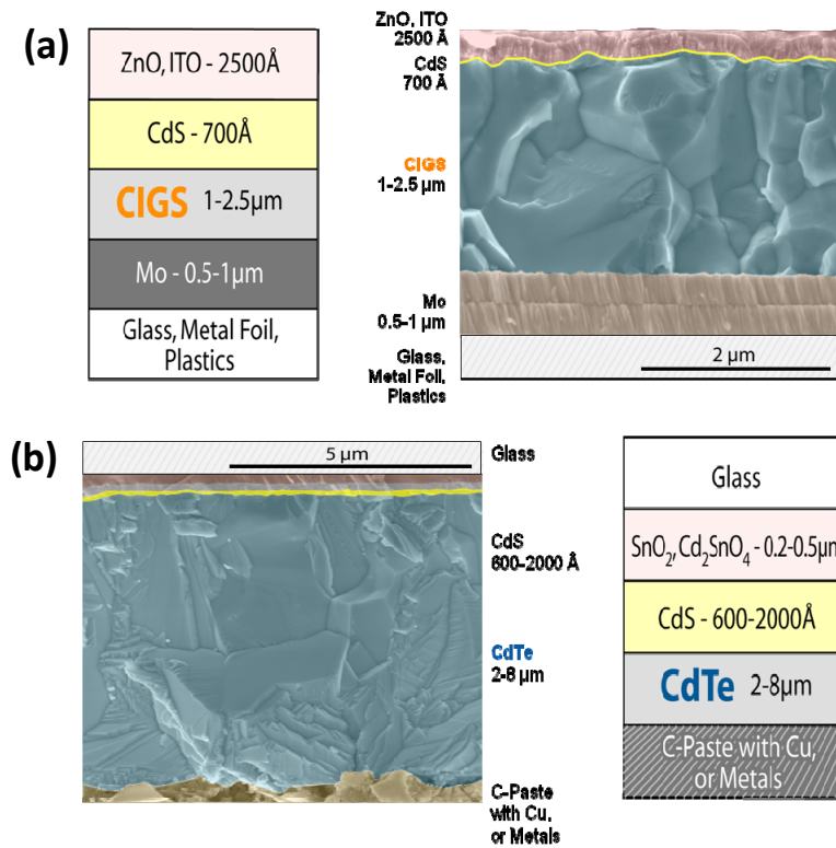
Figure 1.3: The device structures of (a) CIGS substrate solar cell (glass/Mo/CIGS/CdS/ZnO/ITO) and (b) CdTe superstrate solar cell (glass/ \text{SnO}_2\text{:F}/\text{Cd}_2\text{SnO}_4/\text{CdS}/\text{CdTe}/\text{Metals} ). [source: National Renewable Energy Laboratory (NREL)]
