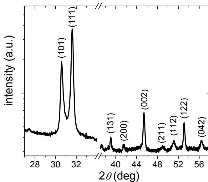
Figure B.3: XRD spectrum of 650 nm-thick SnS films deposited at 70 °C. All peaks match well with Herzenbergite SnS (JCPDS No. 39-0354, a = 4.3291 Å, b = 11.1923 Å, c = 3.9838 Å).
