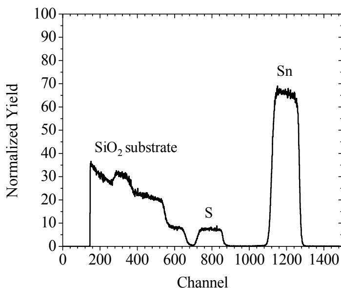
Figure 2.9: A typical RBS spectrum of ALD films deposited at between 100 and 200 °C, indicating stoichiometric SnS to within \pm 1\% .
