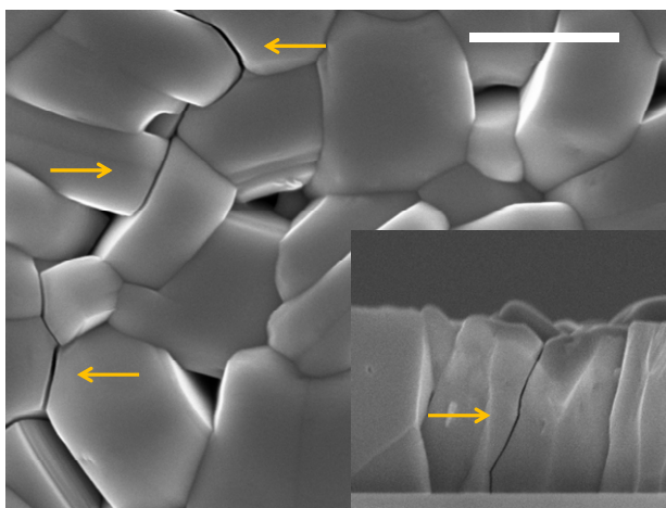
Figure 5.8: a plan-view SEM image of SnS films RTA in \text{H}_2\text{S} above 500 °C showing separation between the surfaces of adjacent grains which propagates into a small crack after cleaving the films. The scale bar is 500 nm.
