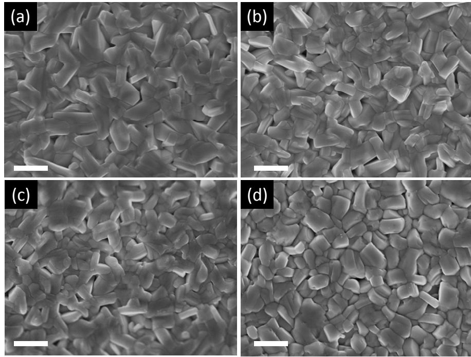
Figure 5.2: SEM images of (a) as-deposited and annealed SnS in 10 Torr of N 2 at substrate temperatures of (b) 300 °C, (c) 350 °C, and (d) 400 °C for 1 hr. The scale bar is 500 nm.
