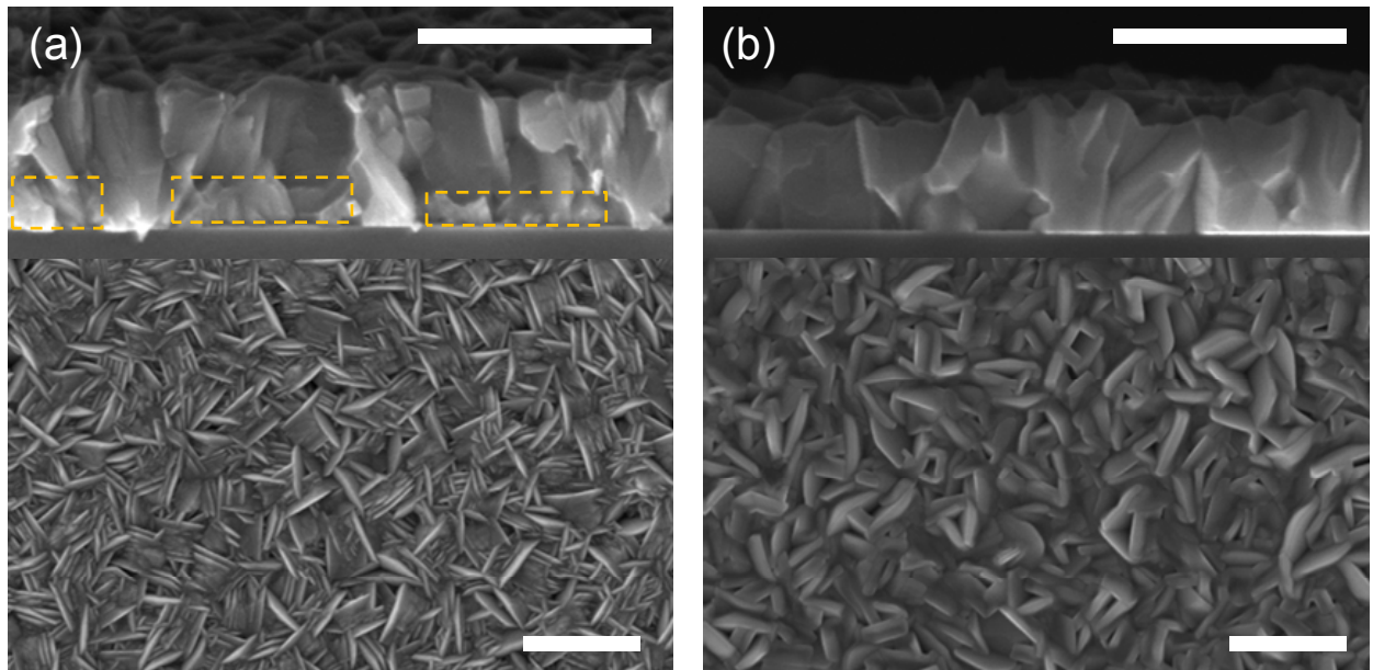
Figure 2.5: Plane-view and cross-sectional (12° tilt) SEM images of SnS films deposited on thermal oxide (SiO 2 ) for 4000 ALD cycles at (a) 120 °C and (b) 200 °C. The boxes in the cross-sectional SEM of (a) indicate the smaller grains formed during the initial film growth. The scale bar is 500 nm.
