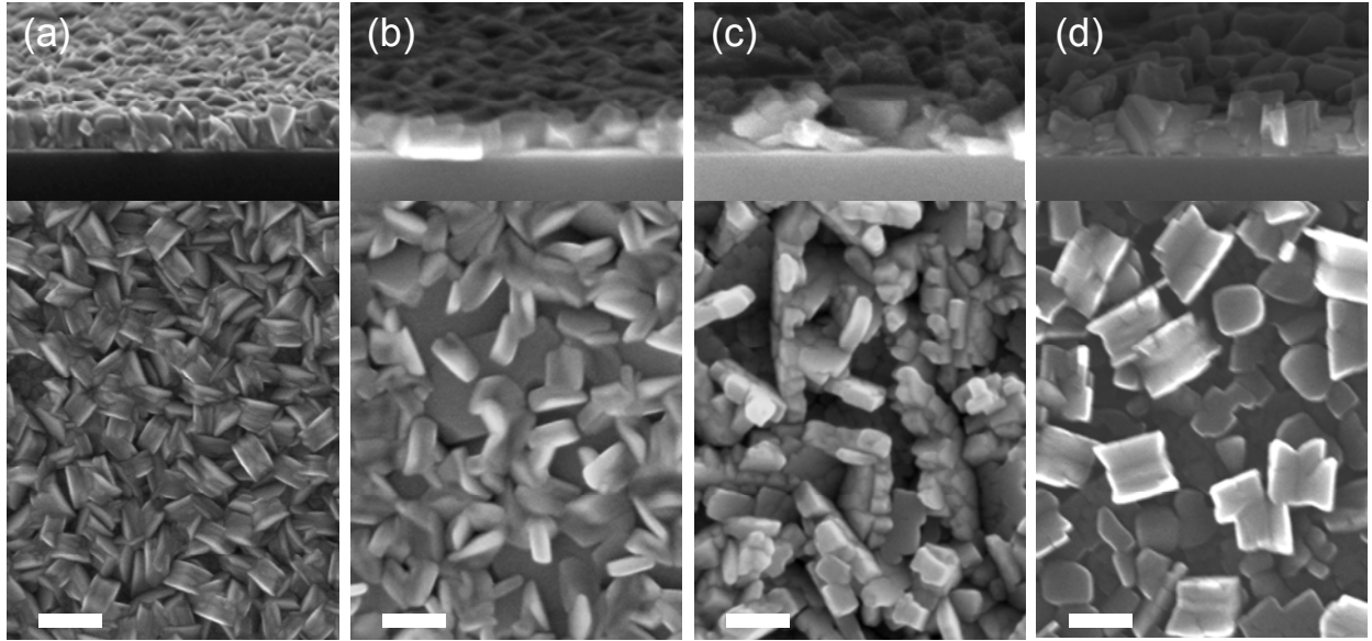
Figure 2.4: Plane-view and cross-sectional (12° tilt) SEM images of SnS films deposited on thermal oxide (SiO 2 ) for 1000 ALD cycles at (a) 120 °C, (b) 200 °C, (c) 250 °C, and (d) 300 °C. The scale bar is 200 nm.
