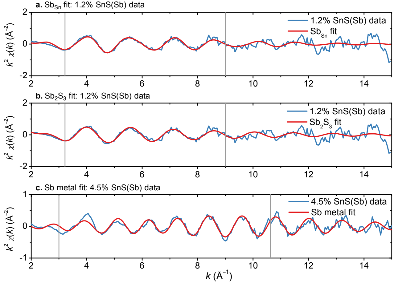
Figure 4.6: EXAFS data and fits for Sb edge: (a) 1.2% SnS(Sb) data with SnS(Sb Sn ) fit, (b) 1.2% SnS(Sb) data with Sb 2 S 3 fit, and (c) 4.5% SnS(Sb) data with Sb metal fit. The vertical lines denote the range chosen for Fourier transformation.
