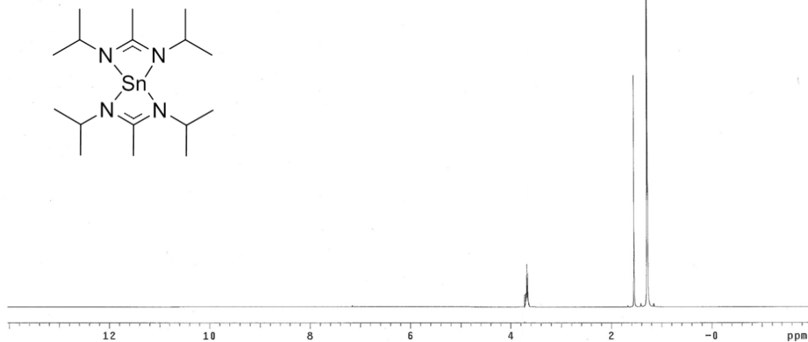
Figure A.3: NMR Spectra (500MHz , \text{C}_6\text{D}_6 ) of bis(N,N'-diisopropylacetamido)tin(II): (a) ^1\text{H} NMR spectrum.
