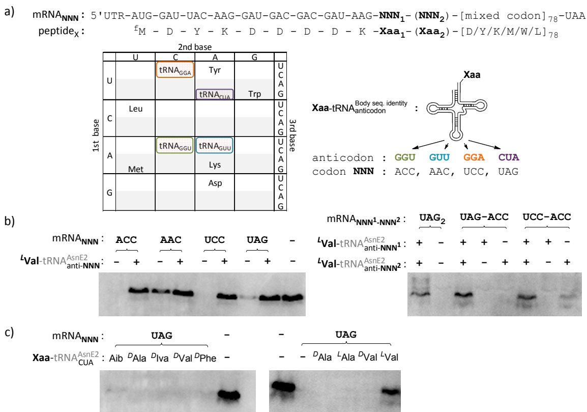
Figure 6. (a) General read-through assay used in this study, peptide with N-term FLAG-tag is expressed followed by one or two unassigned codon NNN and then a stretch of 78mer DYKWLM amino acids. The four anticodons-codon pairs are shown on the right and each tRNA anticodon 's potential decoding range (including wobble) is shown on the left in codon table. (b) Test of aa-tRNA anticodon dependent read-through for four codons ACC, AAC, UCC, UAG and three consecutive dual codons UAG-UAG, UAG-ACC and UCC-ACC. The presence of band of FLAG-containing peptide indicate successful read-through of codons by chemically acylated tRNAs. (c) Test incorporation of several D, L-amino acids. mRNA with label “-” is a template without middle NNN codon and hence full-length peptide synthesis doesn't require chemically acylated
